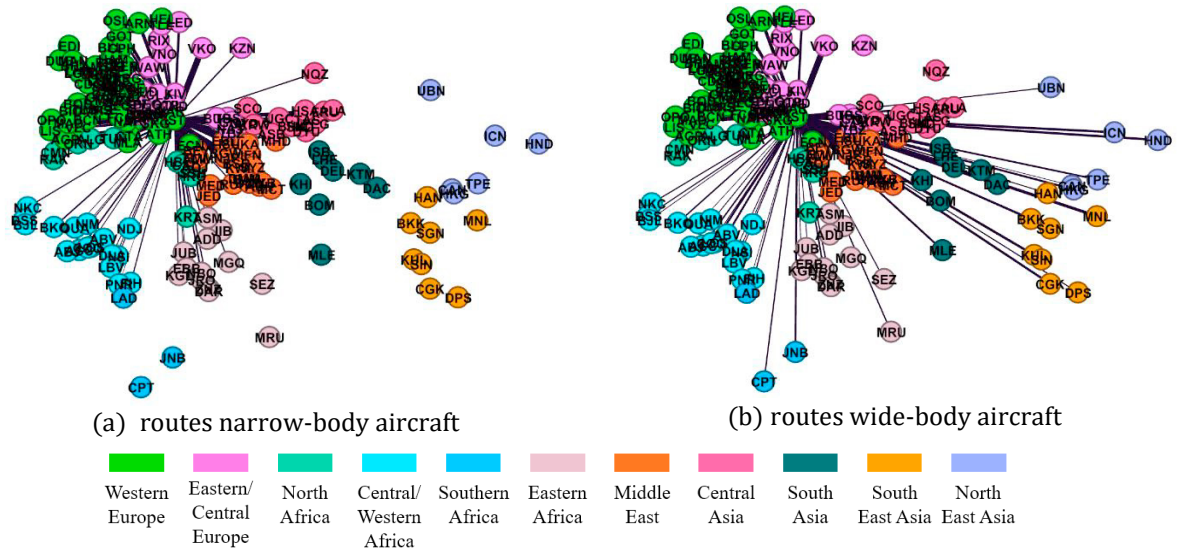
Fig. 6. Narrow-body (a) and wide-body (b) aircraft utilizations in European, African, and Asian regions (thickness and colour represents number of seats offered by respective type of aircraft). In a bigger picture context, as of June 2022, there were total of 154 destinations out of 209 airports globally (about 74%) served by a narrow-body aircraft accounting 52% of all seats and 66% of all flights offered by THY (Source: Author based on data from OAG, 2022).
