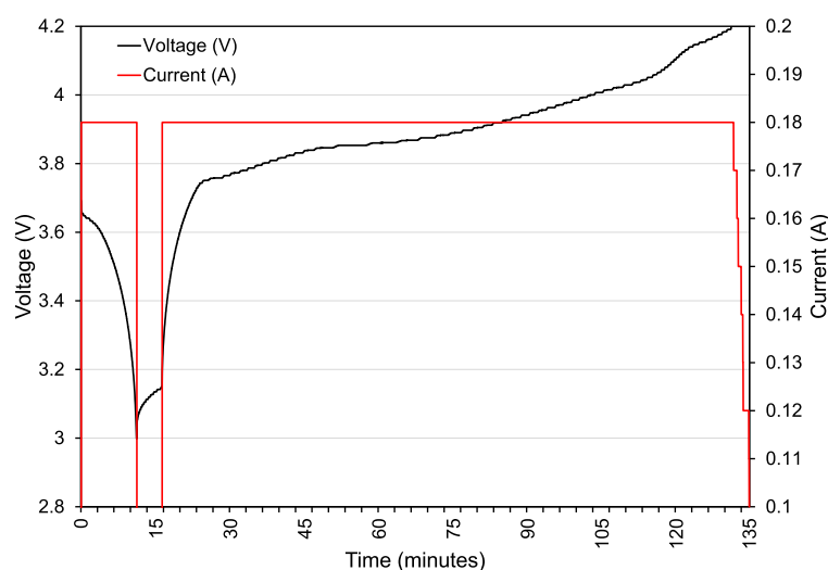
Figure 3. A sample charge–discharge curve.
