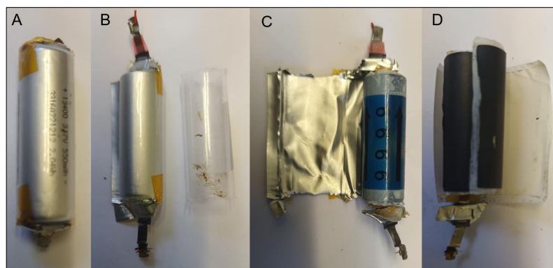
Figure 12. Example of 13400 cell construction: (A) Complete cell, (B) Plastic outer layer, (C) Protective foil casing, and (D) Cell jellyroll construction.
