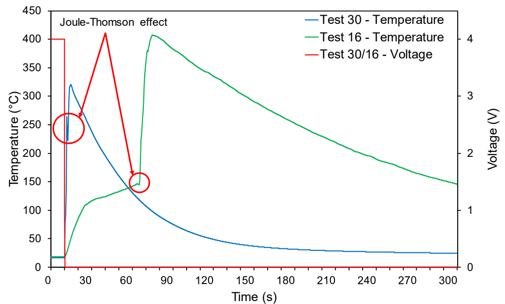
Figure 22. Tests 30 and 16 cell temperature and voltage profile over time.
