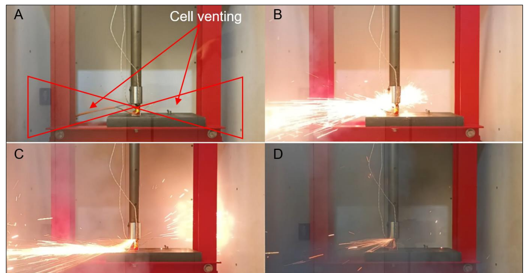
Figure 24. Test 42 cell venting and debris ejection over time: (A) Cell venting, (B) Debris ejection (cell venting + 250 ms), (C) Debris ejection (cell venting + 500 ms), and (D) Debris ejection (cell venting + 750 ms).
