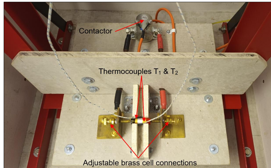
Figure 7. Short-circuit cell holder, electrical connections, and thermocouples.
