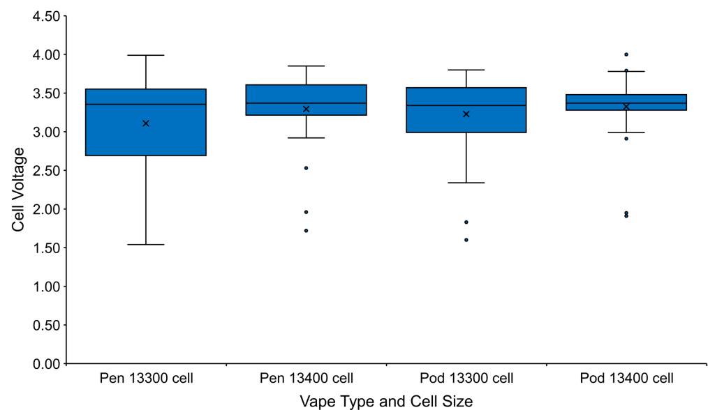
Figure 13. Cell open circuit voltage distribution by vape type and cell.
