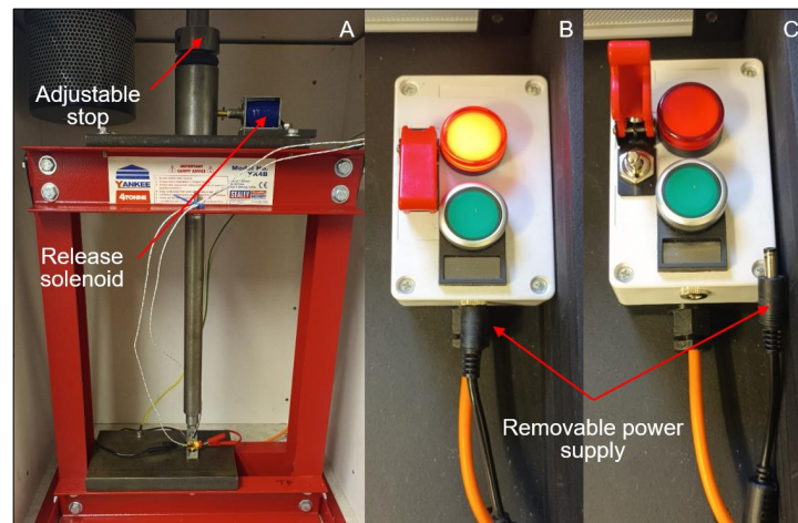
Figure 5. Test rig control systems: (A) mechanical abuse test rig, (B) control system (live), and (C) control system (safe mode).
