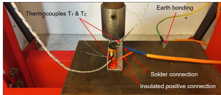
Figure 10. Crush test cell holder, electrical connections, and thermocouples.
