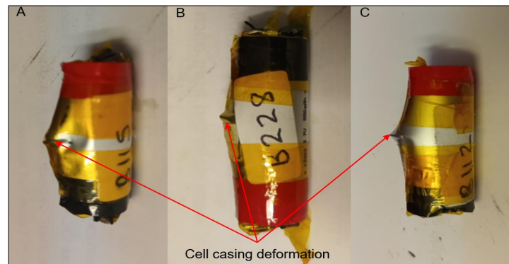
Figure 15. Cell casing central deformation: (A) Test 1—13300 cell 100% SOC, (B) Test 7—13400 cell 50% SOC, and (C) Test 10—13300 cell 50% SOC.
