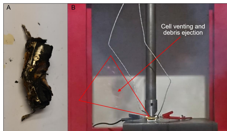
Figure 21. Test 30 cell damage and venting: (A) 13400 cell damage (TR) and (B) Screenshot of cell venting (TR).
