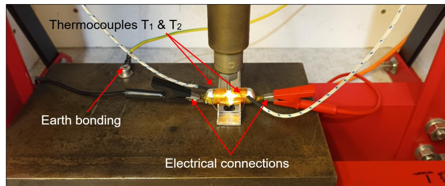
Figure 8. Nail test cell holder, electrical connections, and thermocouples.
