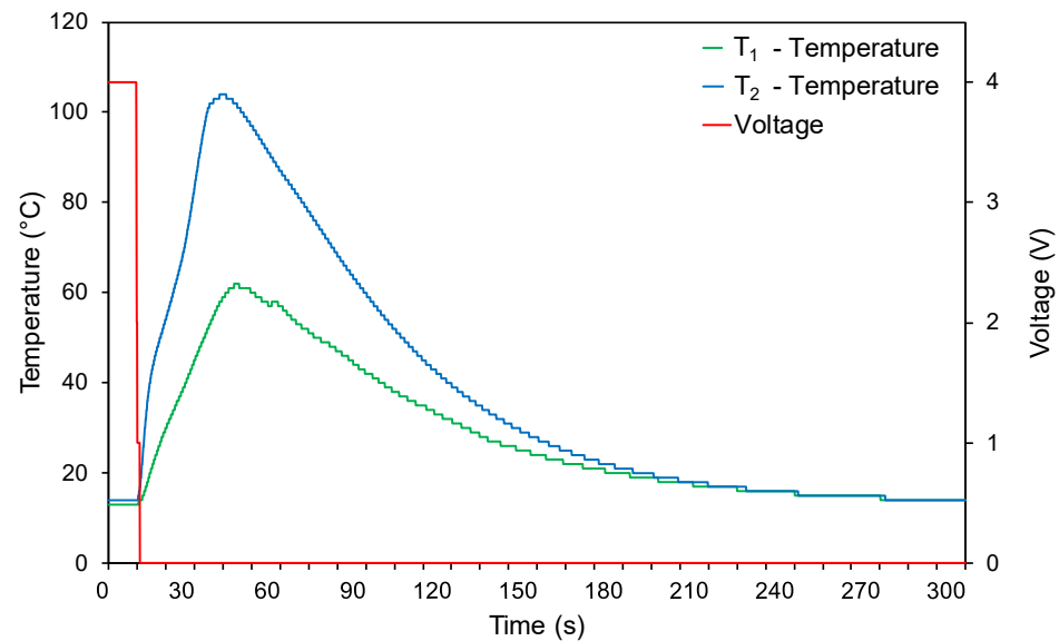
Figure 20. Test 27 cell temperature differential and voltage profile over time.
