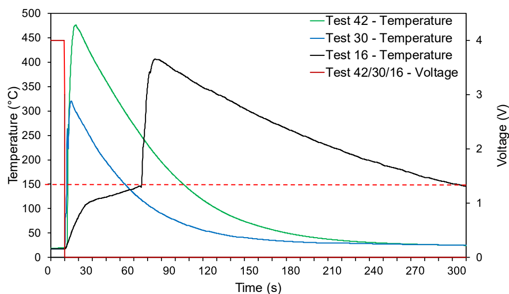
Figure 25. Tests 42, 30, and 16 cell temperature and voltage profile over time.
