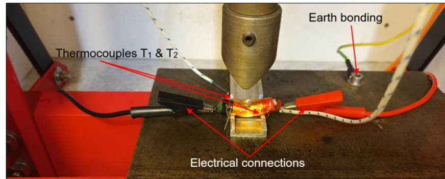
Figure 9. Impact test cell holder, electrical connections, and thermocouples.
