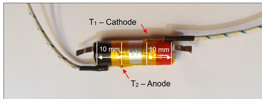
Figure 6. Cell thermocouple positioning.
