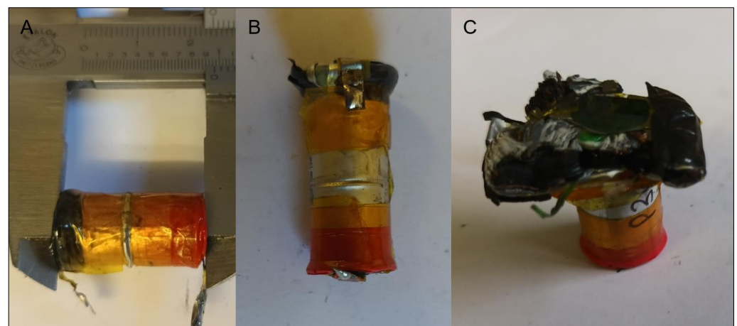
Figure 23. Crush test cell deformation: (A) Test 37—13300 cell—Uniform deformation, (B) Test 48—13400 cell—Uniform deformation, casing ruptured, and (C) Test 41—13400 cell—Significant structural damage.
