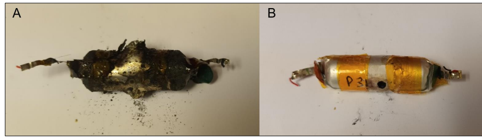
Figure 18. Nail test cell damage comparison: (A) 13400 cell 100% SOC (TR) and (B) 13400 cell 100% SOC.
