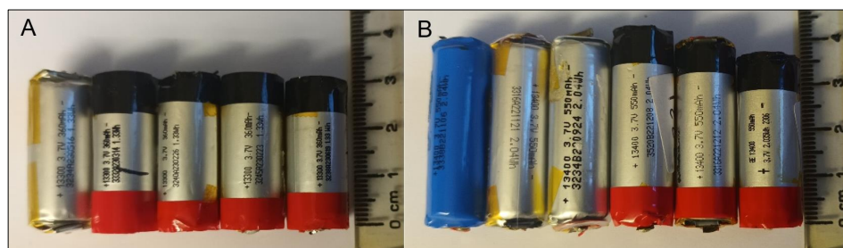
Figure 11. Range of (A) 13300 and (B) 13400 cells removed from SUVs.
