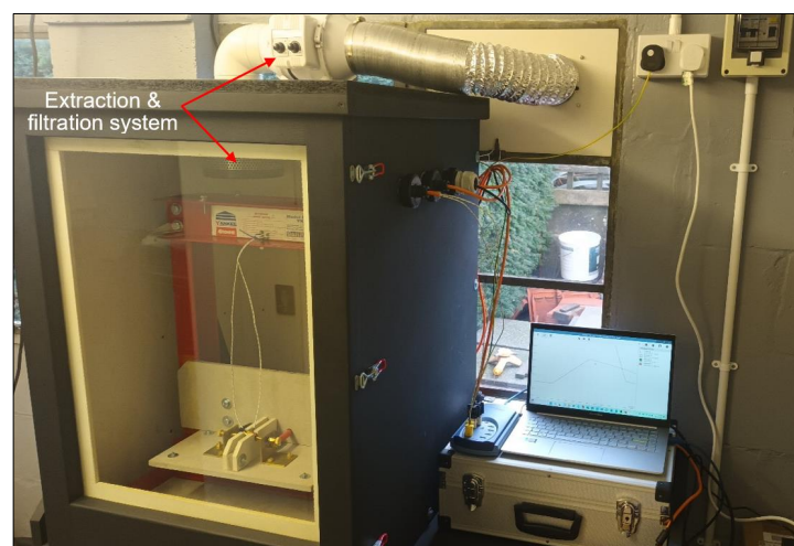
Figure 4. Test rig enclosure, including extraction and filtration system.
