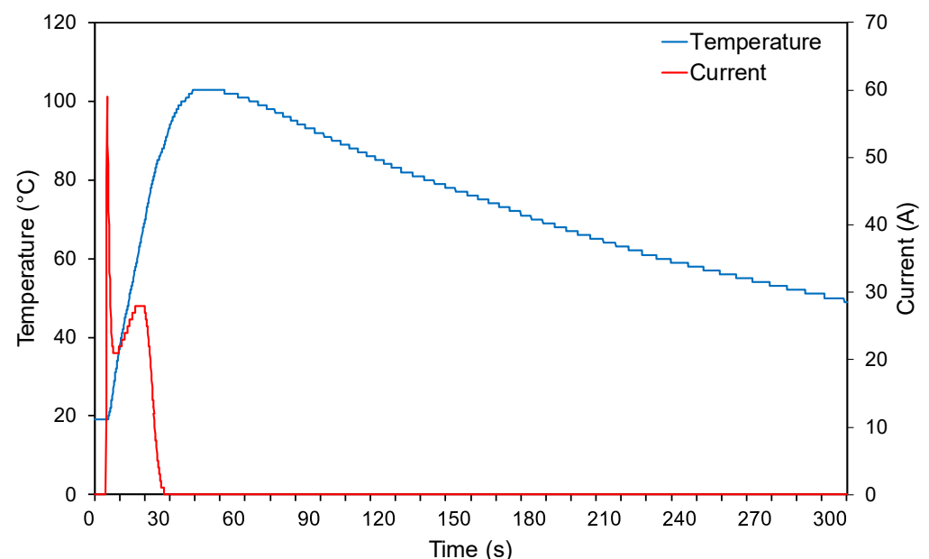
Figure 14. Test 5 cell temperature and current profile over time.
