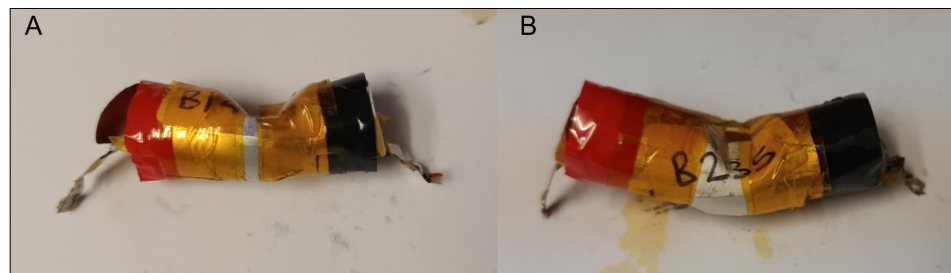
Figure 19. Impact test cell deformation: (A) Test 26—13300 cell and (B) Test 34—13400 cell.
