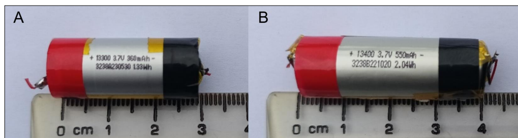
Figure 2. Examples of SUV Li-ion cells: (A) 13300–360 mAh cell and (B) 13400–550 mAh cell.
