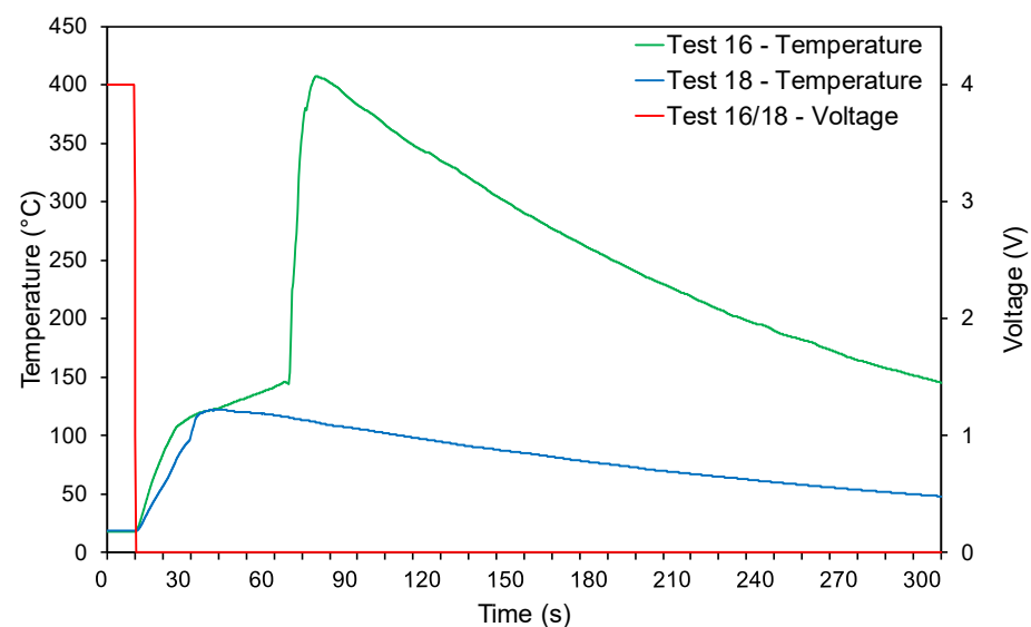
Figure 17. Tests 16 and 18 cell temperature and voltage profile over time.
