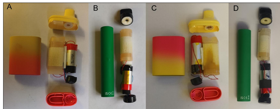
Figure 1. Explode view of pen and pod SUVs: (A) Pod SUV containing 13300–360 mAh cell, (B) Pen SUV containing 13300–360 mAh cell, (C) Pod SUV containing 13400–550 mAh cell, and (D) Pen SUV containing 13400–550 mAh cell.
