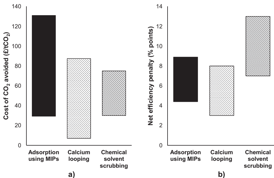
Fig. 5. Comparison of a) economic and b) thermo-economic performance of MIP retrofit scenario with calcium looping and chemical solvent scrubbing retrofits.
