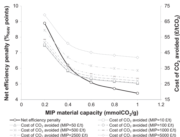
Fig. 6. Effect of MIP sorbent capacity and sorbent cost on the key techno-economic performance indicators.
