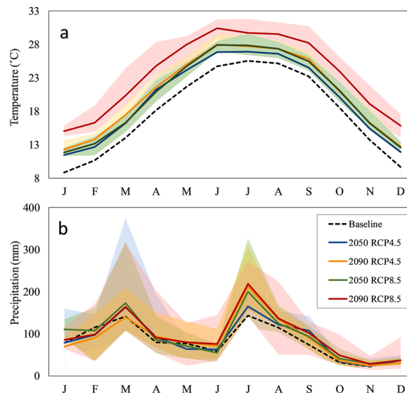
Fig. 4. Monthly means of a) temperature and b) precipitation observed at Bhuntar station for the baseline and the ensemble means of bias corrected outputs of the selected climate models in RCP4.5 and RCP8.5 for the middle and the end of the century. Shading corresponding to the line data denotes the ensemble range of projections within five GCMs.
