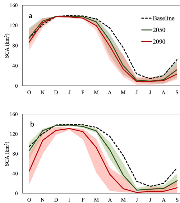
Fig. 5. Simulated mean monthly SCA (km 2 ) in the catchment till the end of century under a) RCP4.5 and b) RCP8.5. The lines indicate the ensemble mean and the shading denotes the range of WEAP outputs for runs forced with five GCMs projections.
