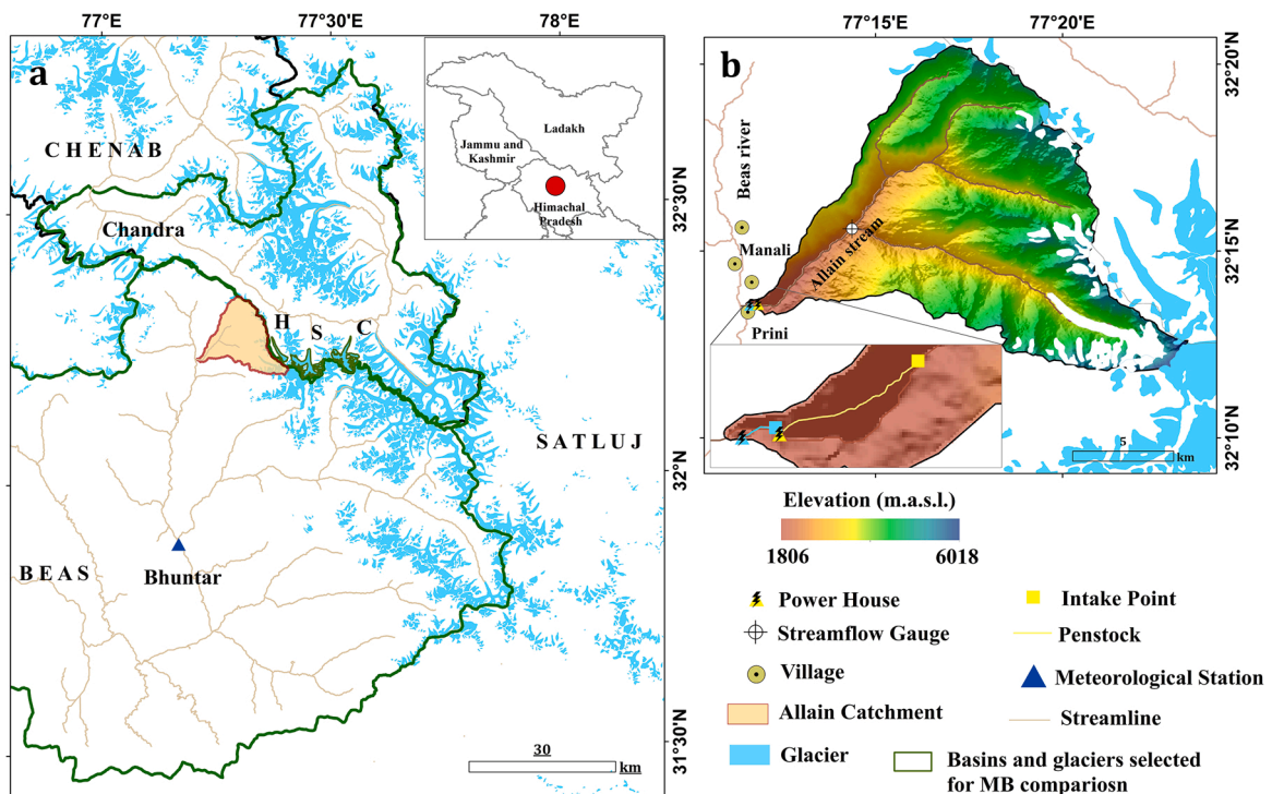
Fig. 1. Location map of the study area. Panel a shows location of Allain catchment in Beas basin along with the meteorological station Bhuntar. Additional basins (Beas and Chandra) and individual glaciers (Hamtah, Sakchum and Chhota Shigri denoted as H, S and C, respectively) selected for comparative mass balance estimates are located adjacent to Allain catchment (Table S1). Panel b shows Allain catchment on ASTER DEM along with locations of the streamflow gauge and nearby towns of Manali and Prini. The inside box shows the close-up of the powerhouses of Aleo-1 (Yellow) and Aleo-2 (Blue) plants with intake points and penstocks.
