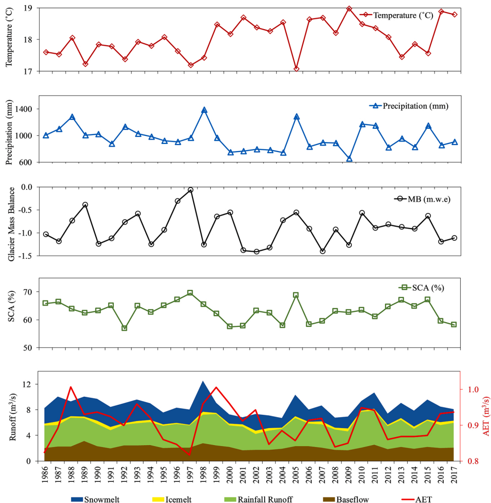
Fig. 2. Interannual variation in the streamflow contributions and actual evapotranspiration (AET) ( \text{m}^3/\text{s} ) at the catchment outlet, mean simulated SCA (% of the total catchment area) and glacier MB (m.w.e.) in the catchment, and mean annual temperature and precipitation observed at Bhuntar observatory.
