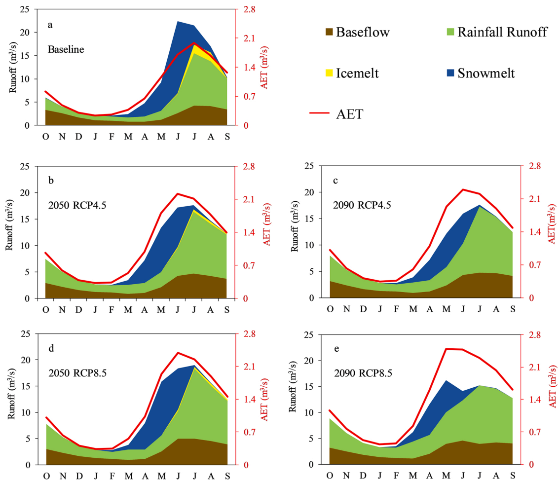
Fig. 6. Mean monthly streamflow components (snowmelt runoff, icemelt runoff, rainfall-runoff and baseflow) and AET until the end of the century for RCP4.5 and 8.5. The values are the ensemble mean of WEAP outputs considering the projections of five GCMs.
