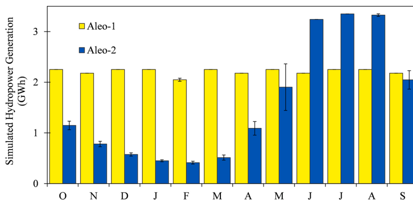
Fig. 3. Simulated average monthly hydropower generation (GWh) at Aleo-1 and Aleo-2 Hydropower projects. Average for Aleo-1 is from 2005–2018 whereas for Aleo-2 is taken from 2014–2018 based on the start of the operation of the projects. Error bars indicate the inter-annual variation.
