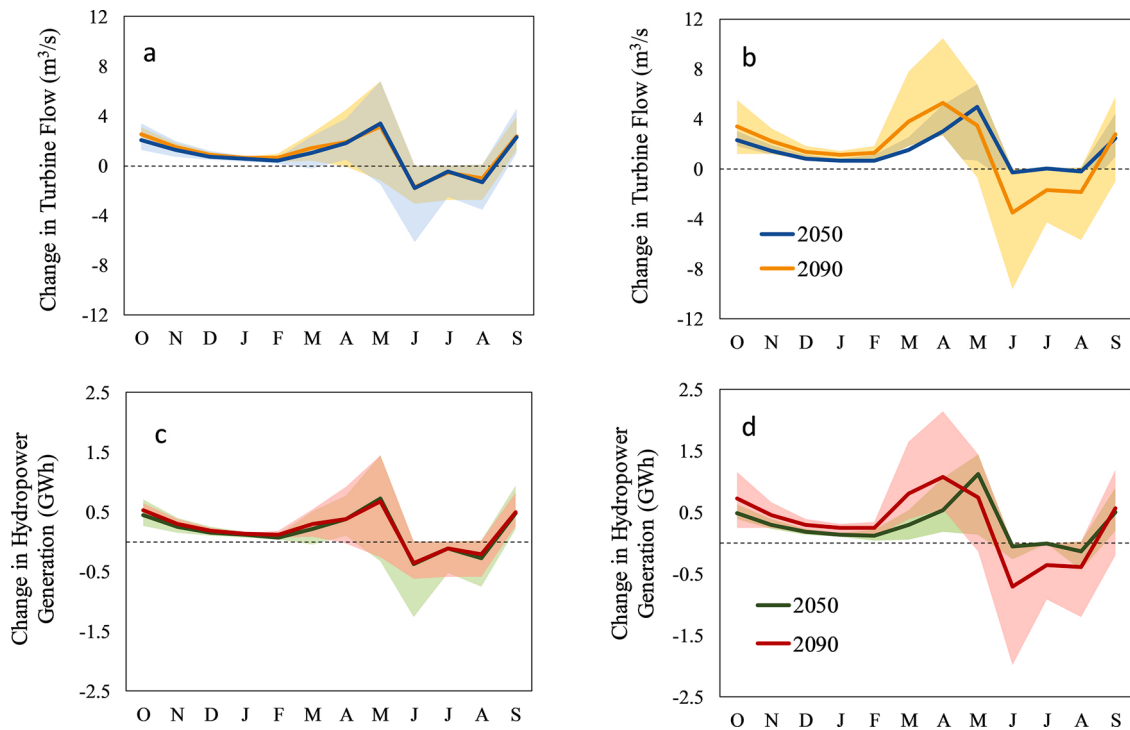
Fig. 8. Panel a and b show changes in mean monthly turbine flow ( \text{m}^3/\text{s} ) in RCP4.5 and RCP8.5, respectively. Panel c and d show change in mean monthly hydropower production (GWh) at Aleo-2 power project compared to the baseline for RCP4.5 and RCP8.5, respectively. Lines indicate the ensemble means while the shading indicates the ensemble range of WEAP outputs considering the projections of five GCMs.
