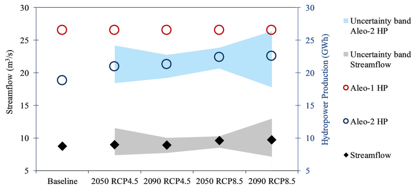
Fig. 7. Projected average annual streamflow ( \text{m}^3/\text{s} ) and hydropower production (GWh) at Aleo-1 and Aleo-2 power projects until the end of the century; the values are the ensemble mean and the shading shows the range of WEAP outputs for runs forced with five GCMs projections.
