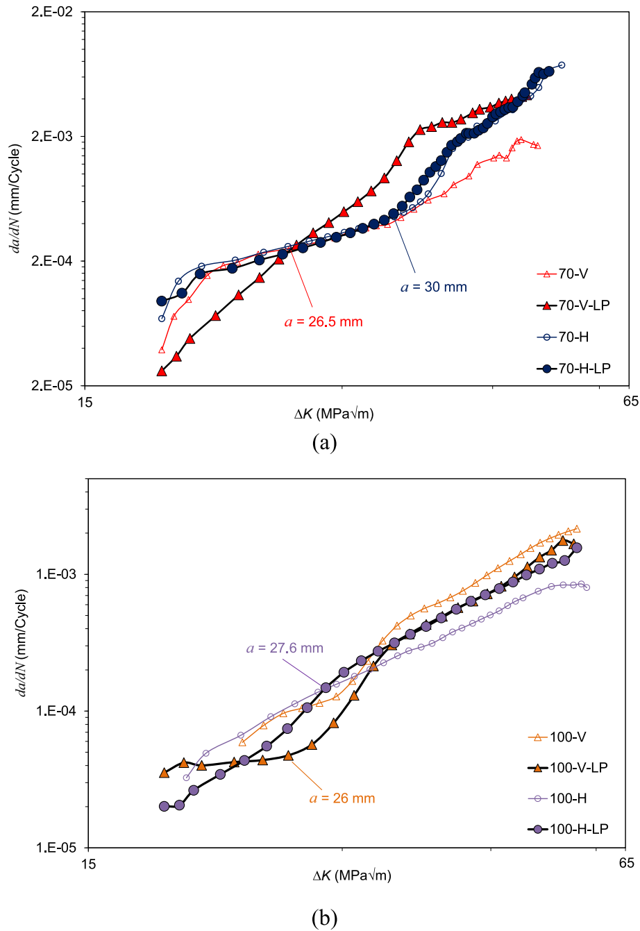
Fig. 8. Comparison of CFCG rates from WAAM specimens with and without LP surface treatment for (a) ER70S-6, and (b) ER100S-1 materials.
