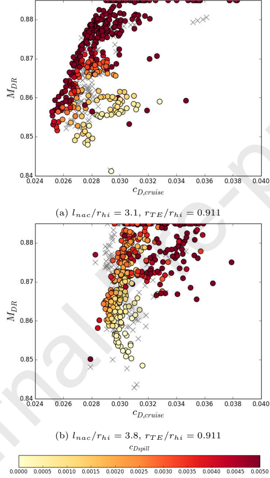
Figure 6: Pareto optimal sets for optimisations performed at two different lengths with pressure limitations ( C_{shock} , C_{inflect} ), plotted as a function of the performance metrics (o), with the Pareto sets from the optimisations without pressure limitations shown in grey (x)
