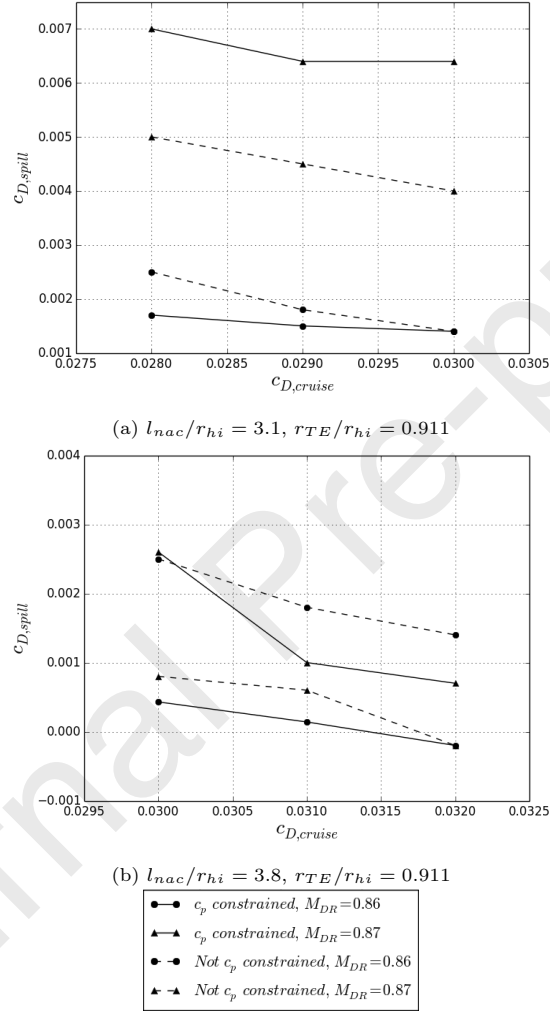
Figure 7: Minimum achievable c_{Dspill} for different nacelle lengths and different required levels of c_{Dcruise} and M_{DR}
