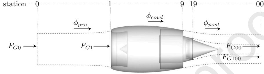
Figure 1: Thrust and drag accounting system
