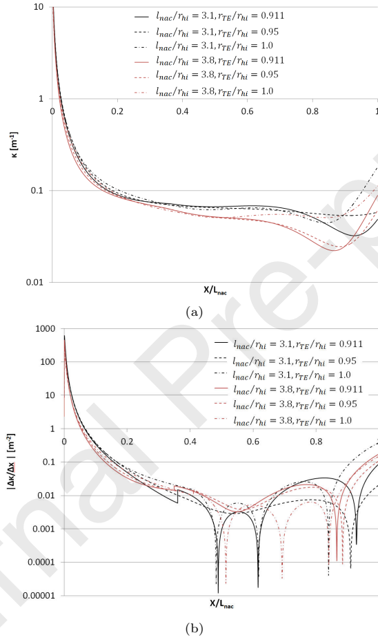
Figure 14: (a) Curvature distribution and (b) Rate of change of curvature distribution for six chosen optimal designs for different lengths and trailing edge radii
