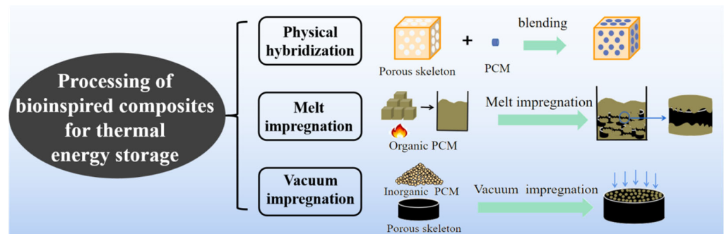
Figure 6. Processing of bioinspired composites for thermal energy storage.
