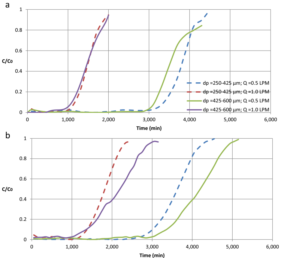
Fig. 5 Impact of particle size and gas flow rate on the breakthrough curve. a Pelletized limestone. b Natural limestone. Flow rates at 1 barg and 20 °C
