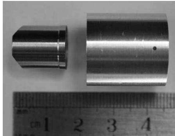
Fig 7 Sabot design 3, aluminium pot.
