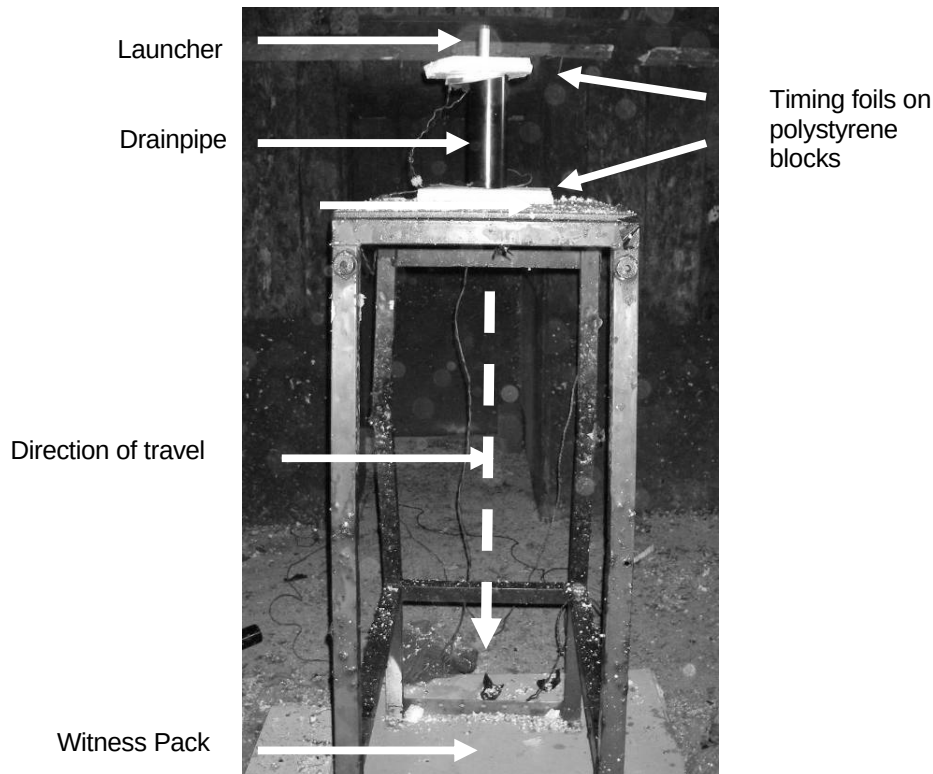
Fig 4 General layout of the explosive launch method.
