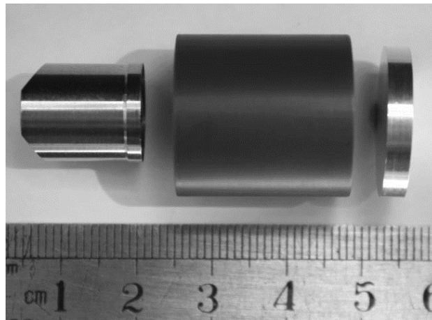
Fig 6 Sabot design 2, PVC pot.
