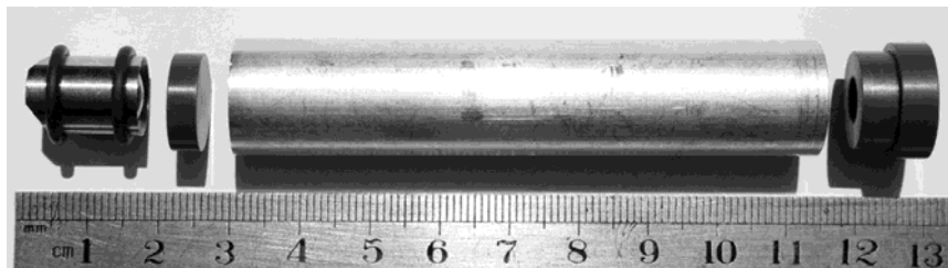
Fig 2 Disassembled components of the explosive launcher
