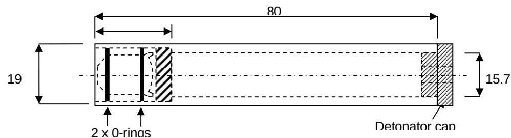
Fig 3 Explosive launcher general layout, (dimensions in mm).
