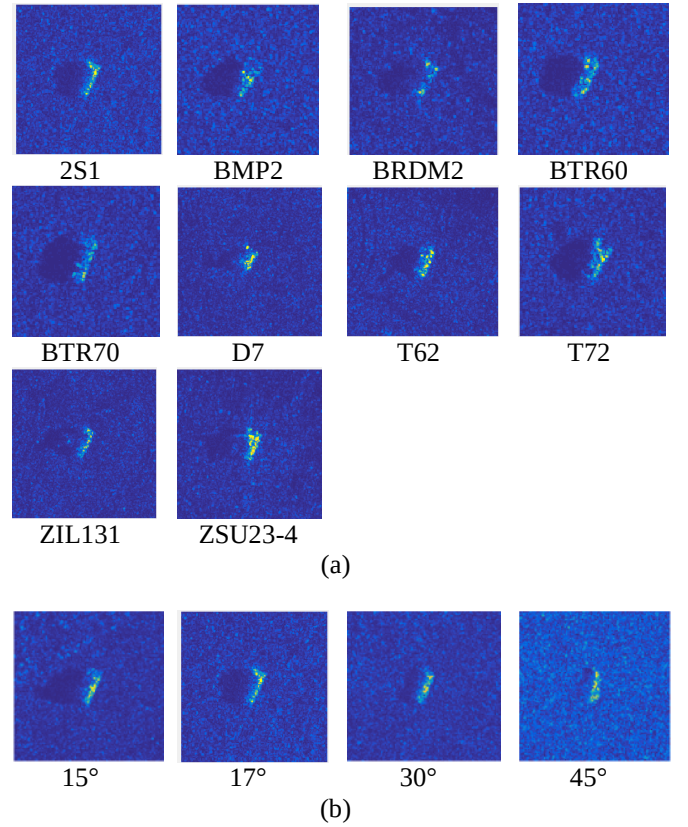
Figure 3: (a) 10 classes of the public MSTAR database at 17° depression angle (b) the 2S1 target at various depression angles while at same azimuth
