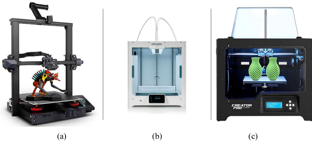
Fig. 14. Popular FDM- and FFF-based 3D printers in the market, with open and enclosed systems: (a) Creality Ender 3 (credit: Creality Ender) [110], (b) Ultimaker S5 (credit: Ultimaker) [111], and (c) Flashforge Creator Pro 3D (credit: Flashforge) [112].
