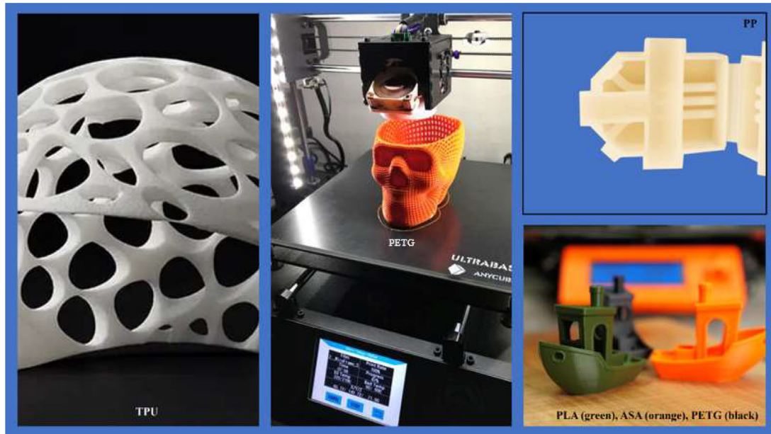
Fig. 6. Some modelling and functional parts made of thermoplastic and elastomeric materials (e.g. TPU, PETG, PP, PLA and ASA) produced using extrusion-based AM (adapted from [52–55]).
