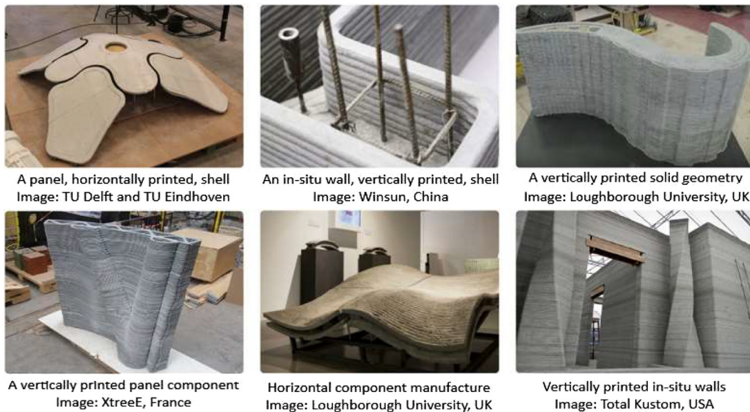
Fig. 11. Concrete structures produced by different groups using extrusion-based AM (reprinted with permission from Ref. [78])
