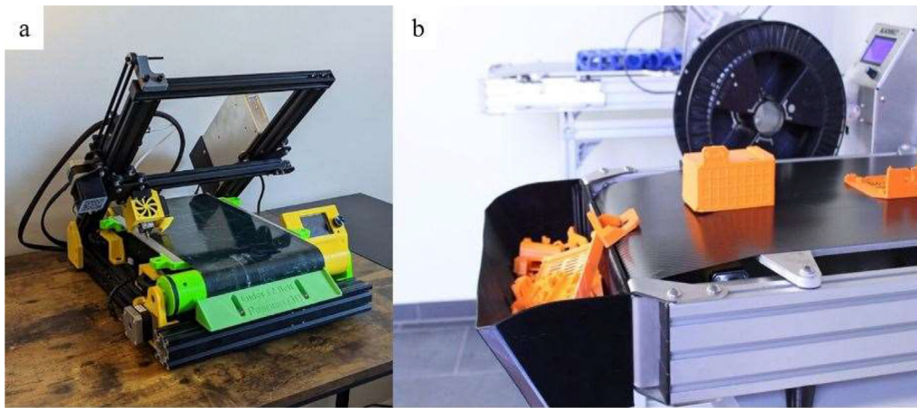
Fig. 16. Representations of some popularly used FDM- and FFF-based 3DP machines: (a) Conveyor 3D Printer (credit: Powerbelt3D) [127], and (b) Conveyor 3D printer conveying printed parts into a collection unit [128] to allow for continuous printing, and thereby eliminating stops usually used for part removal and printing restarts.
