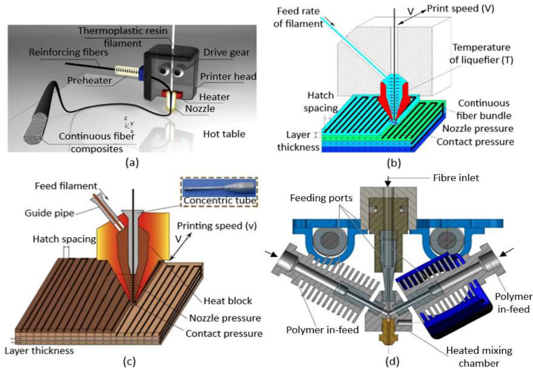
Fig. 7. Some of current extrusion-based AM machine setups for fabrication of polymer composite parts: (a) Namiki et al. [58]; (b) Tian et al. [59]; (c) Ye et al. [60]; (d) Prüß and Vietor [61] (adapted with permission from Ref. [62]).
