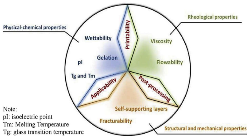
Fig. 12. Material properties to consider upon extrusion-based AM of structures and parts (reprinted with permission from Ref. [101]).
