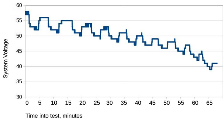
Figure 6. eKub battery system voltage against time, during conduct of ground test shown in Fig. 5.
