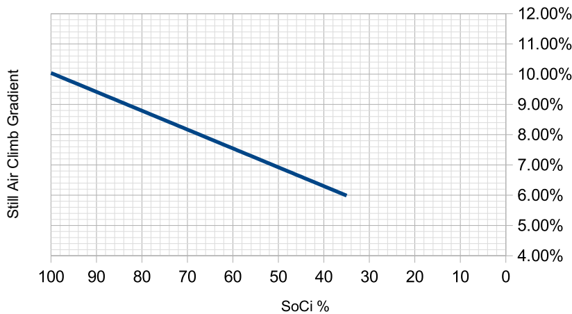
Figure 15. eKub standardised climb gradient between 0 and 1,000ft sHd versus SoC I .
