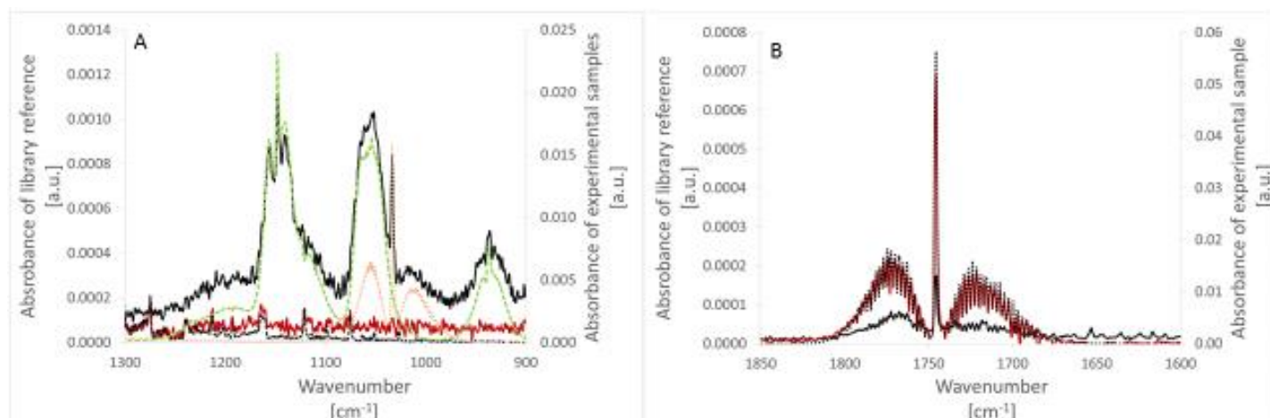
Figure 2. FTIR spectra of a formaldehyde in hydrogen standard after different storage times, held at ambient temperature. Figure 2A presents the FTIR spectra in wavelength area 1300-900 \text{cm}^{-1} . This spectral region presents the characteristic absorptions from the C-O bond in the methanol and dimethoxymethane fingerprint. Figure 2B presents FTIR spectra in wavelength area 1850-1600 \text{cm}^{-1} . This spectra region presents the carbonyl stretch of formaldehyde. The red line correspond to formaldehyde in hydrogen after 1 day of production. The solid black line correspond to formaldehyde in hydrogen after 1 year. The grey dotted line corresponds to the formaldehyde reference spectrum; the green dotted line to the dimethoxymethane reference spectrum and the yellow dotted line to the methanol reference spectrum. All reference spectra are taken from the PNNL database.
