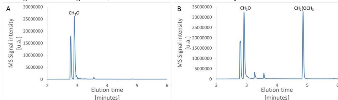
Figure 4. GC-MS with preconcentrator chromatograms for mixture B. The Figure 3A presents the chromatogram of mixture B after preparation (aged 1 day). Only one compound is present, CH 2 O. The Figure 3B presents the chromatogram of mixture B after 80 days of storage at room temperature. Three species were identified using the mass spectra: CH 2 O, CH 3 OH and CH 2 (OCH 3 ).
