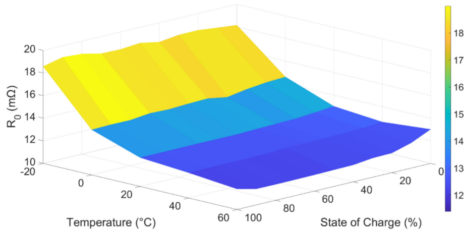
Fig. 9. 3D representation of R_0 versus SOC and temperature.
