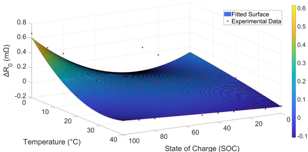
Fig. 18. Fitted surface for \Delta R_0 with experimental points.
