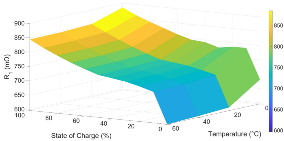
Fig. 12. 3D representation of R_1 , SOC and temperature.
