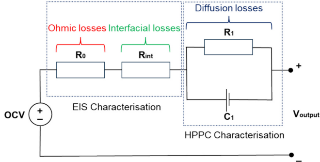
Fig. 4. Schematic of the ECM.
