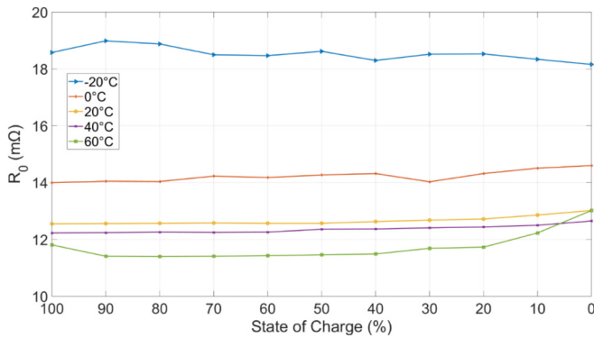
Fig. 7. R_0 plot against SOC values for -20 °C, 0 °C, 20 °C, 40 °C and 60 °C.
