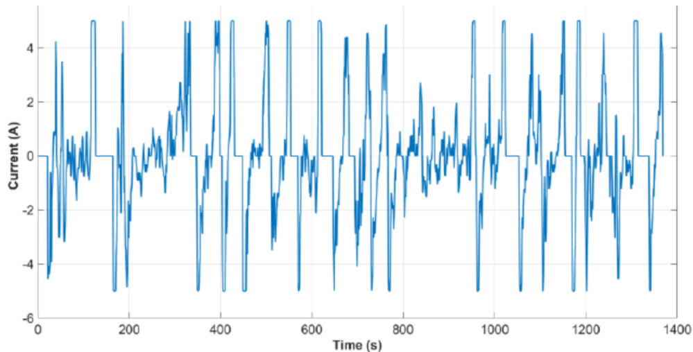
Fig. 20. Dynamic current profile for model validation.
