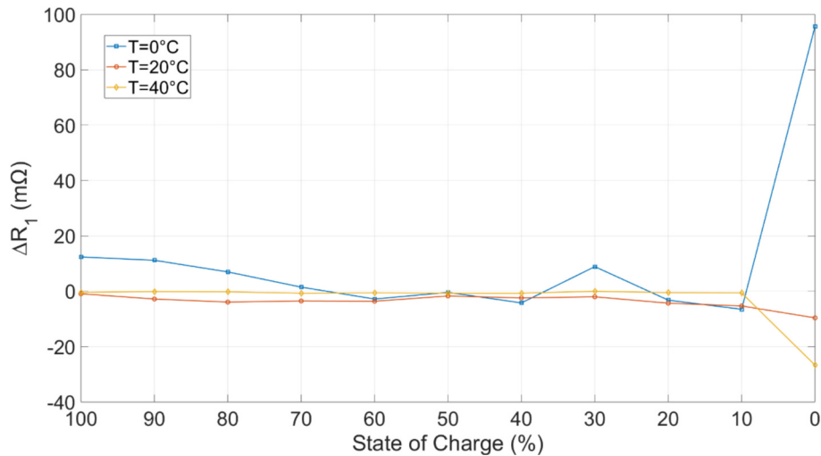
Fig. 16. \Delta R_1 plot against SOC for T = 0^\circ\text{C} , T = 20^\circ\text{C} and T = 40^\circ\text{C} .
