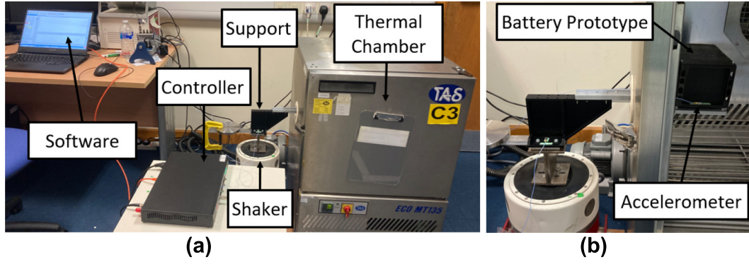
Fig. 2. (a) Overall vibration testing setup. (b) battery prototype and accelerometer inside the chamber.
