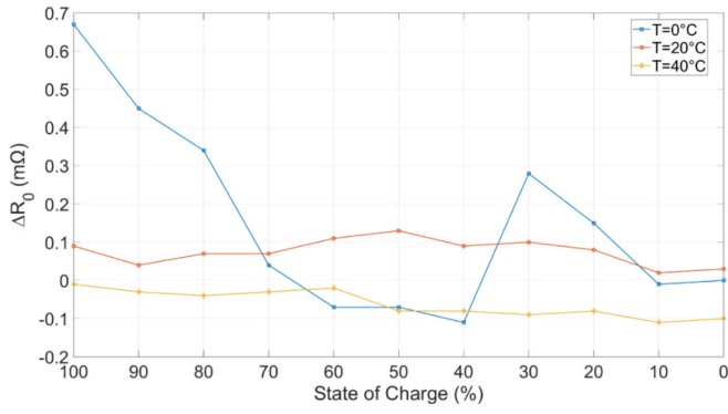
Fig. 14. Resistance's variation \Delta R_0 with respect to SOC and temperature.
