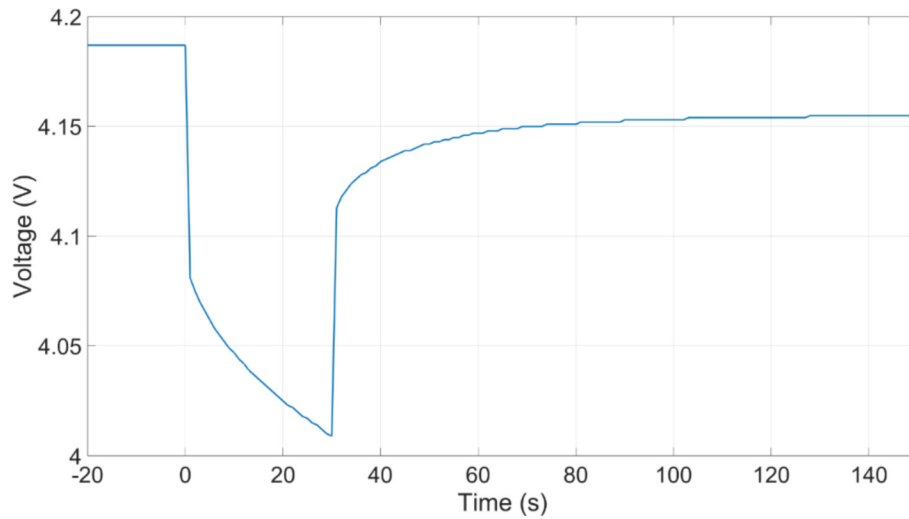
Fig. 11. Voltage response at 20 °C and 100% SOC.
