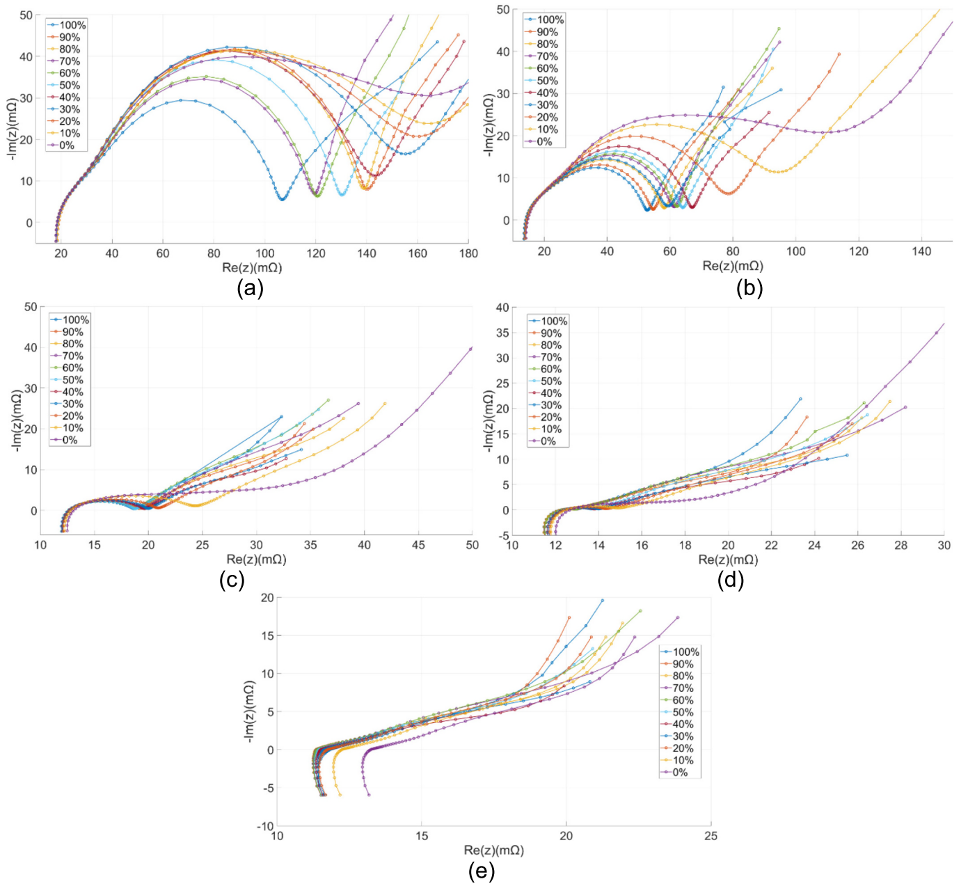
Fig. 6. Nyquist plots against for (a) -20 °C, (b) 0 °C, (c) 20 °C, (d) 40 °C and (e) 60 °C.
