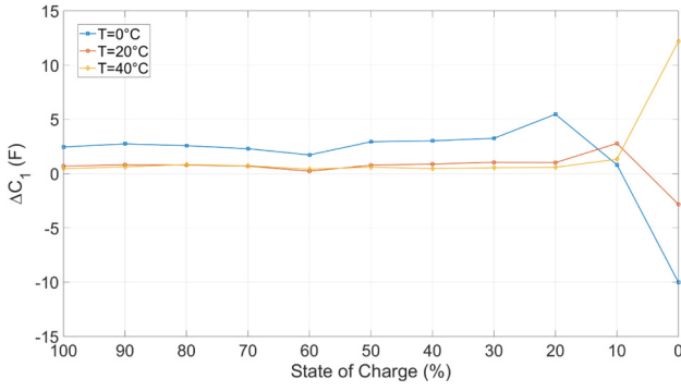
Fig. 17. \Delta C_1 plot against SOC for T = 0^\circ\text{C} , T = 20^\circ\text{C} and T = 40^\circ\text{C} .
