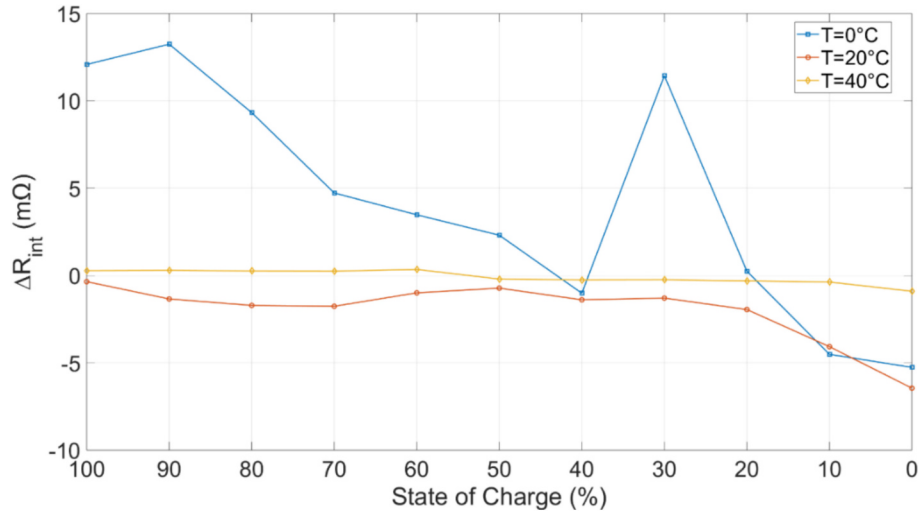
Fig. 15. Resistance's variation \Delta R_0 with respect to SOC and temperature.
