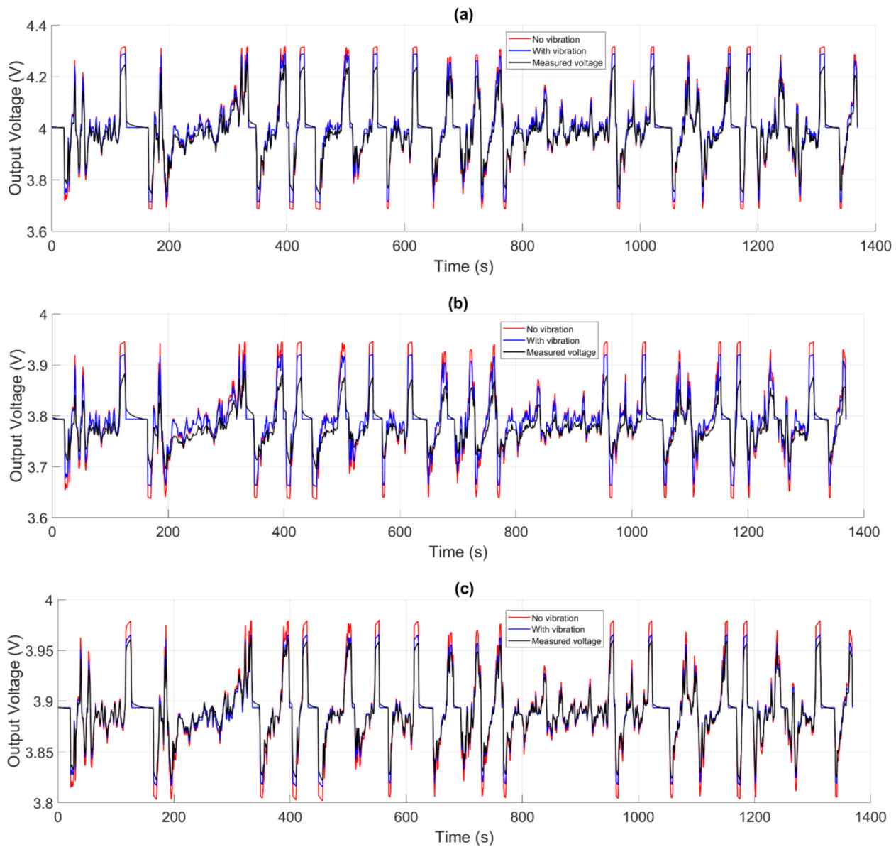
Fig. 21. Voltage output comparison between the experimental cell and the ECM considering without and with vibration influence. (a) at 10 °C and 85% SOC. (b) at 25 °C and 65% SOC. (c) at 35 °C and 75% SOC.
