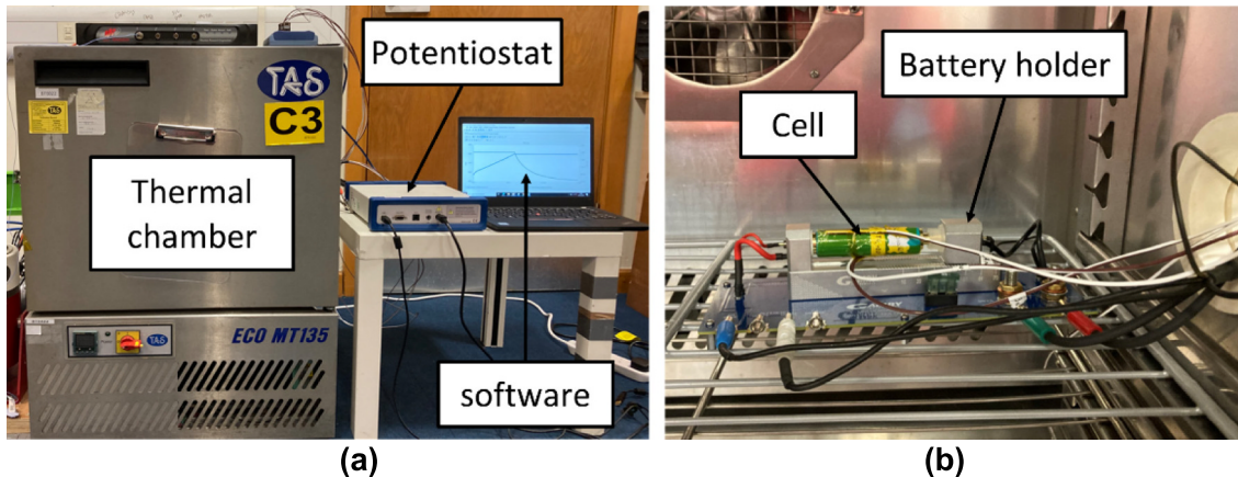
Fig. 1. (a) Thermal chamber, potentiostat and software. (b) Battery holder and cell inside the thermal chamber.
