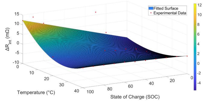
Fig. 19. Fitted surface for \Delta R_{\text{int}} with experimental points (b).
