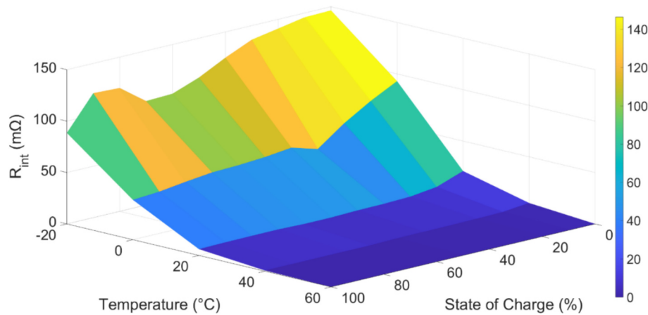
Fig. 10. 3D representation of R_{\text{int}} versus SOC and Temperature.
