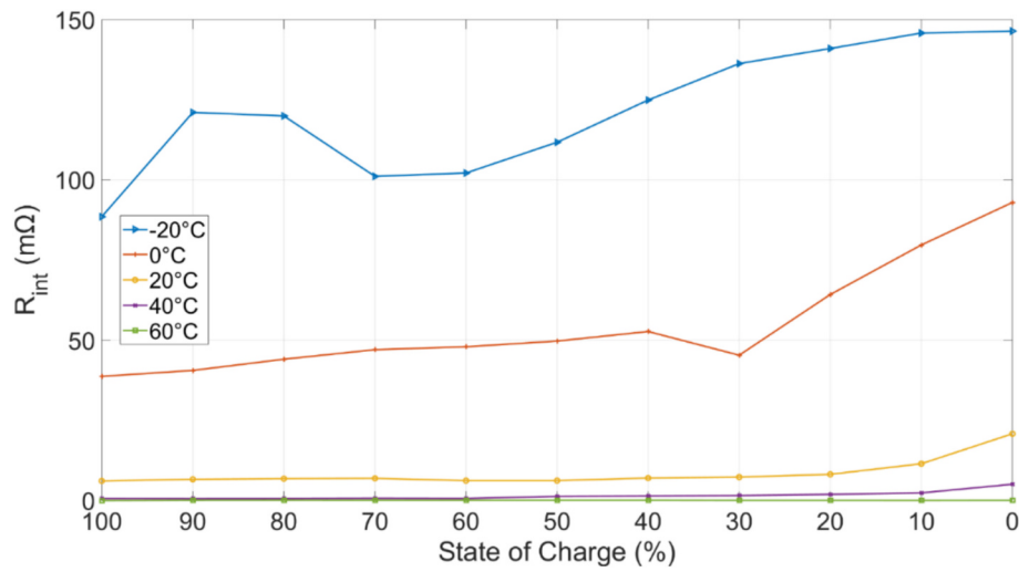
Fig. 8. Rint plot against SOC values for -20\text{ }^{\circ}\text{C} , 0\text{ }^{\circ}\text{C} , 20\text{ }^{\circ}\text{C} , 40\text{ }^{\circ}\text{C} and 60\text{ }^{\circ}\text{C} .
