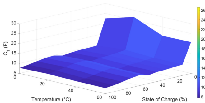
Fig. 13. 3D representation of C_1 , SOC and temperature.
