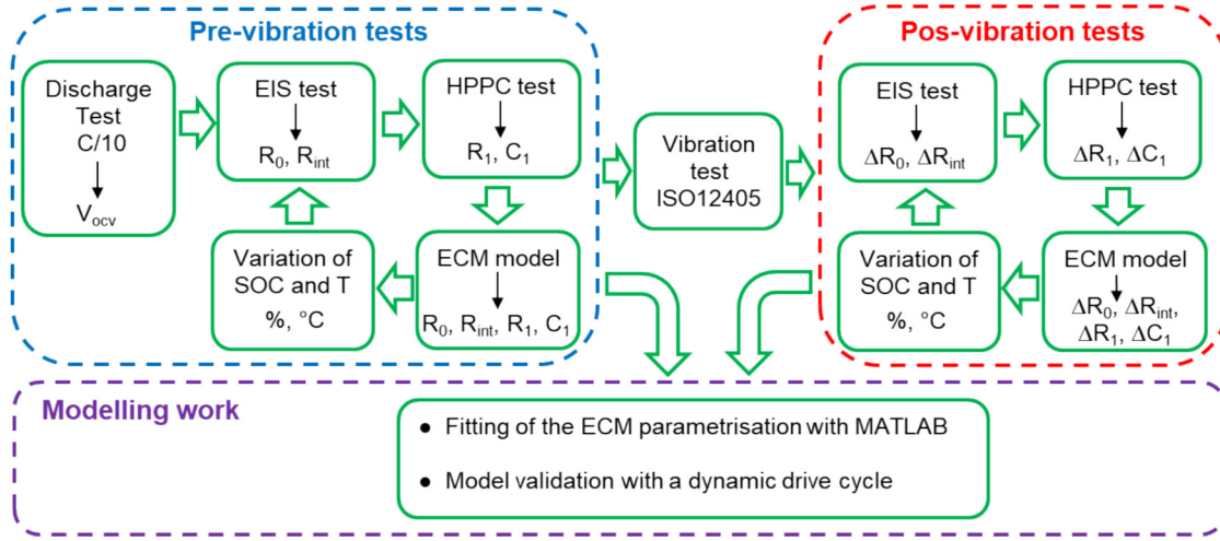
Fig. 3. Schematic of experiments.
