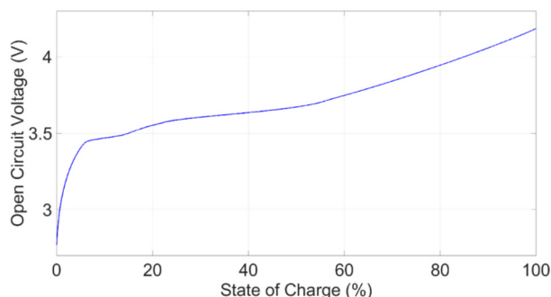
Fig. 5. OCV-SOC curve.
