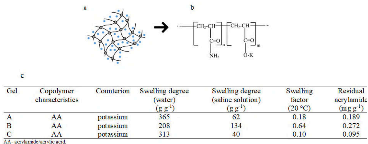
Figure 1. a. Representation of copolymer swollen in water. The lattice represents the cross-linking and the grey circles the hydrogel cross-linking points. The blue circles represent the water molecules inside the hydrogel. b. Structural representation of acrylamide and potassium acrylate copolymer. c. description of the hydrogels used in this study.
