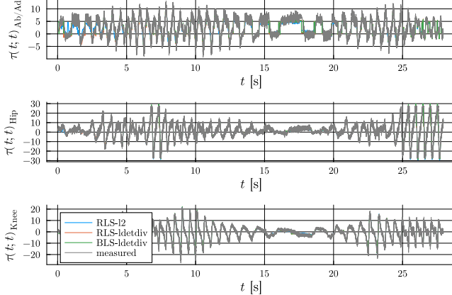
Fig. 2. Measured and Predicted Joint Torques ( f_s = 10^3 Hz)
