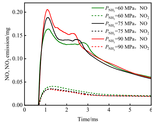
Figure 19. NO and NO 2 emissions with different P_{\text{NH}_3} .
