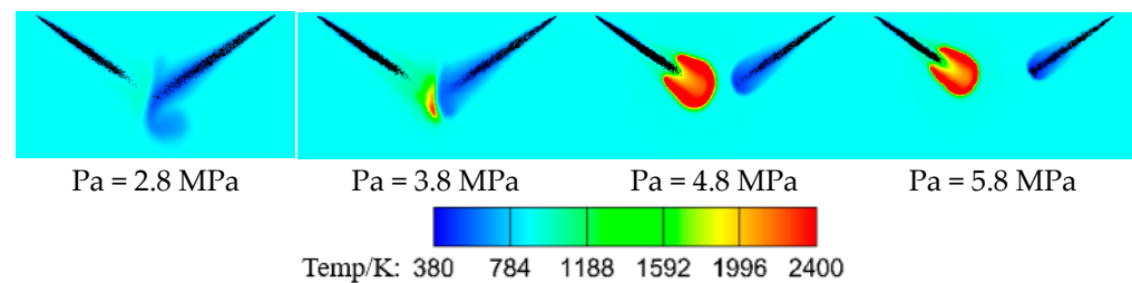
Figure 21. Temperature at ignition moment at different P_a .
