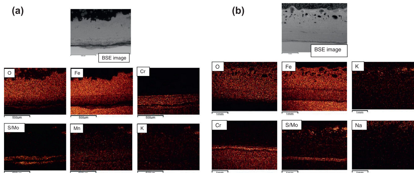
Fig. 8. BSE image and X-ray maps of cross-section through (a) bare T92 alloy and (b) covered in deposit D1 exposed to simulated oxy-fired combustion gases (with 6260 vppm \text{SO}_2 /1700 vppm HCl) at 700 °C for 1000 h.
