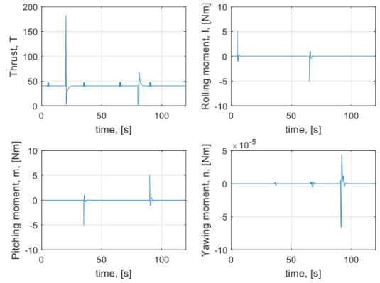
Fig. 3. Time history of virtual command
