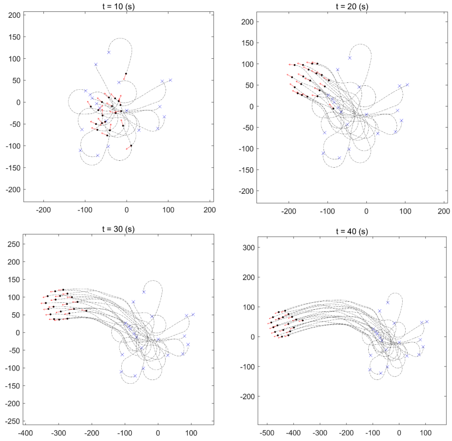
Figure 11: Trajectory of the fully active group in the fully connected network.
