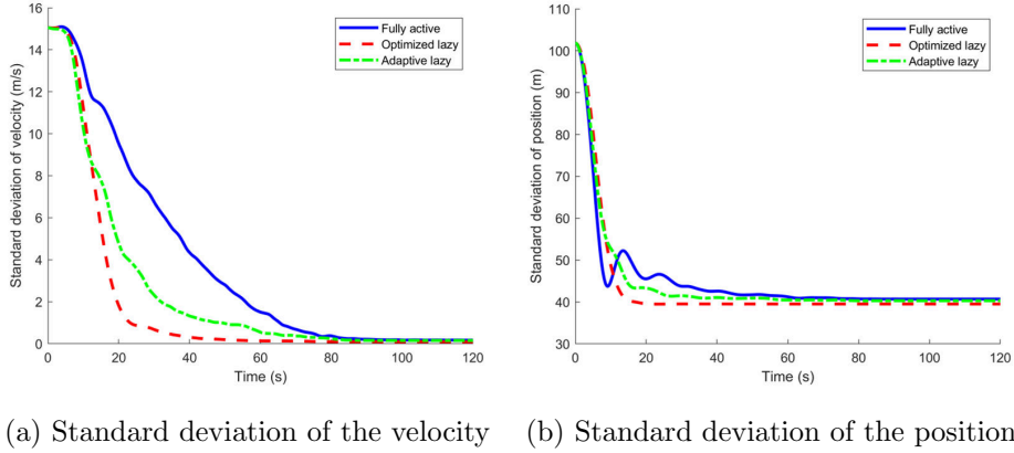
Figure 21: Comparison of standard deviations in the adaptive inactiveness approach.
