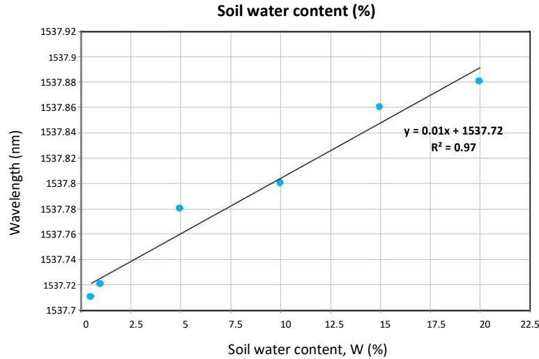
Figure 4. Wavelength (nm) vs. Soil water content (%)
