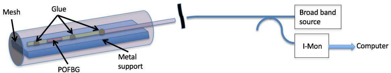
Figure 1. Sensor construction
