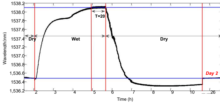
Figure 2. The measured/reflect wavelength from the POF sensor for 20% soil moisture content at 20.5°C
