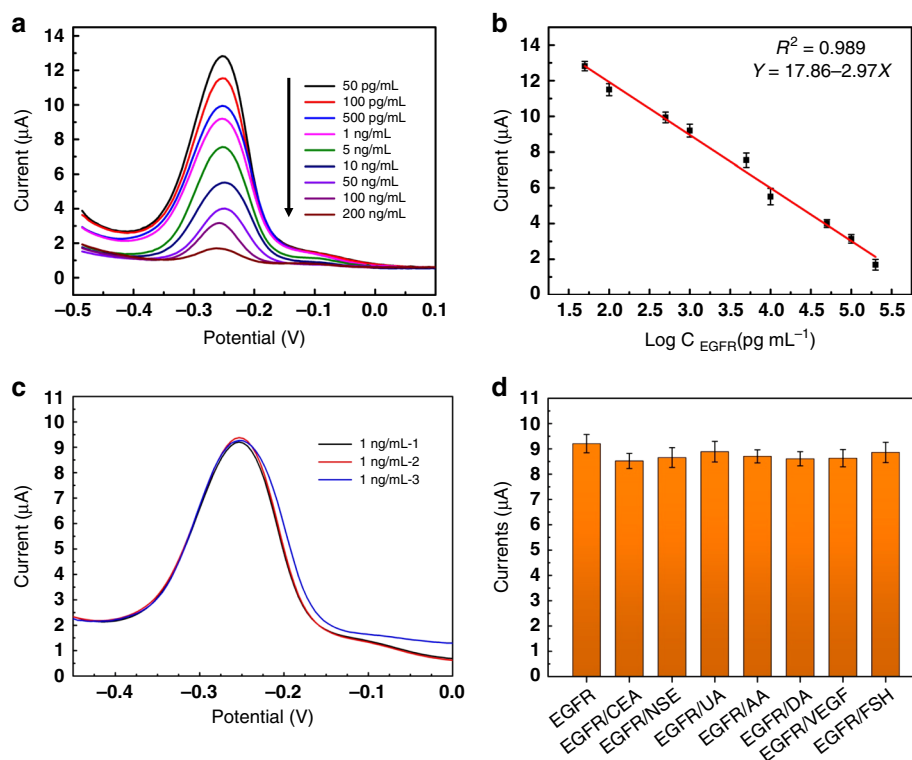
Fig. 6 Assay results of standard EGFR solutions in 0.1 M PBS (pH = 7.4). a DPV responses of the origami-paper-based aptasensor to different concentrations of standard EGFR solutions ranging from 0.05 ng mL -1 to 200 ng mL -1 ; b peak current of DPV response as a function of the concentration of EGFR; c three repeated measurements of 1 ng mL -1 of EGFR; d selectivity of the aptasensor to 1 ng mL -1 of EGFR, and 1 ng mL -1 of EGFR mixed with 10 ng mL -1 solutions of some potentially interfering substances, carcinoembryonic antigen (CEA), neuron-specific enolase (NSE), uric acid (UA), ascorbic acid (AA), dopamine (DA), vascular endothelial growth factor (VEGF), and follicle-stimulating hormone (FSH). Error bars in c and d are standard deviations over three independent measurements
