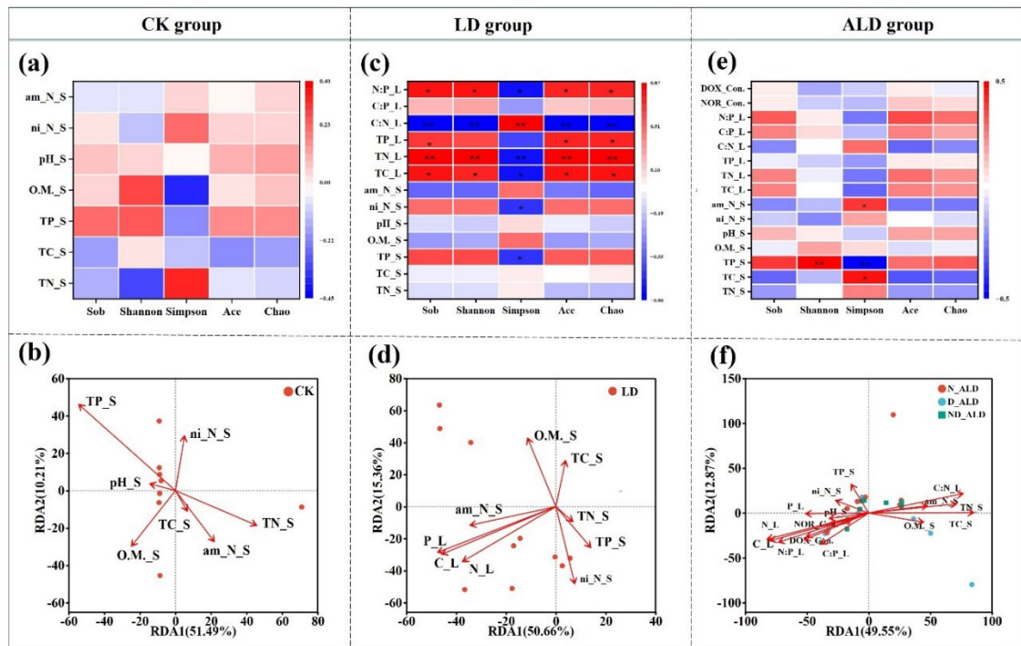
Fig. 6 Heatmap correlation at the phylum level between the bacterial community Alpha diversity and physicochemical properties, and Redundancy analysis (RDA) at the OTU level between the bacterial community structure and the physicochemical properties. (a and b: control group (CK); c and d: litter decomposition group (LD); e and f: antibiotic-litter decomposition group (ALD); * P < 0.05 ; ** P < 0.01 ; *** P < 0.001 )
