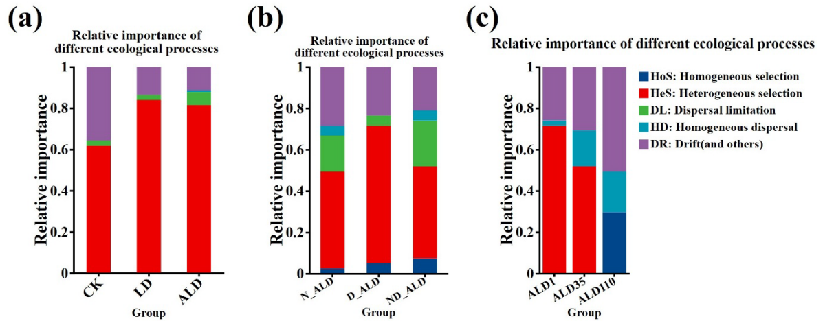
Fig. 5 The assembly processes of sediment microbial communities. (a: Control group (CK), litter decomposition group (LD), and antibiotic-litter decomposition group (ALD); b: norfloxacin-litter decomposition group (N-ALD), doxycycline-litter decomposition group (D-ALD), a combination of both antibiotics-litter decomposition group (ND-ALD); c: three decomposition times of three antibiotic-litter decomposition groups)
