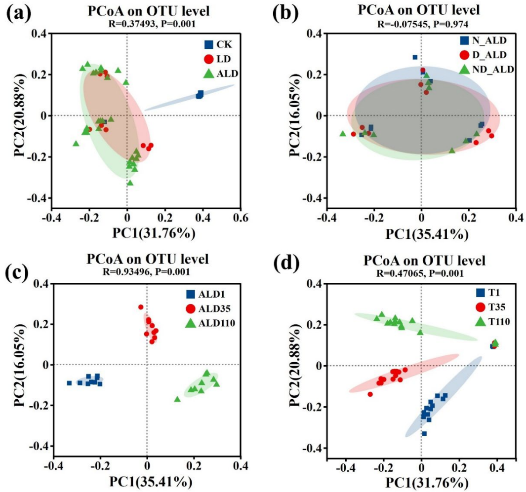
Fig. 2 Principal co-ordinate analysis (PCoA) of the bacterial community structure. (a: Control group (CK), litter decomposition group (LD), and antibiotic-litter decomposition group (ALD); b: norfloxacin-litter decomposition group (N-ALD), doxycycline-litter decomposition group (D-ALD), a combination of both antibiotics-litter decomposition group (ND-ALD); c: three decomposition times of three antibiotic-litter decomposition groups; d: three decomposition times across all experimental groups)
