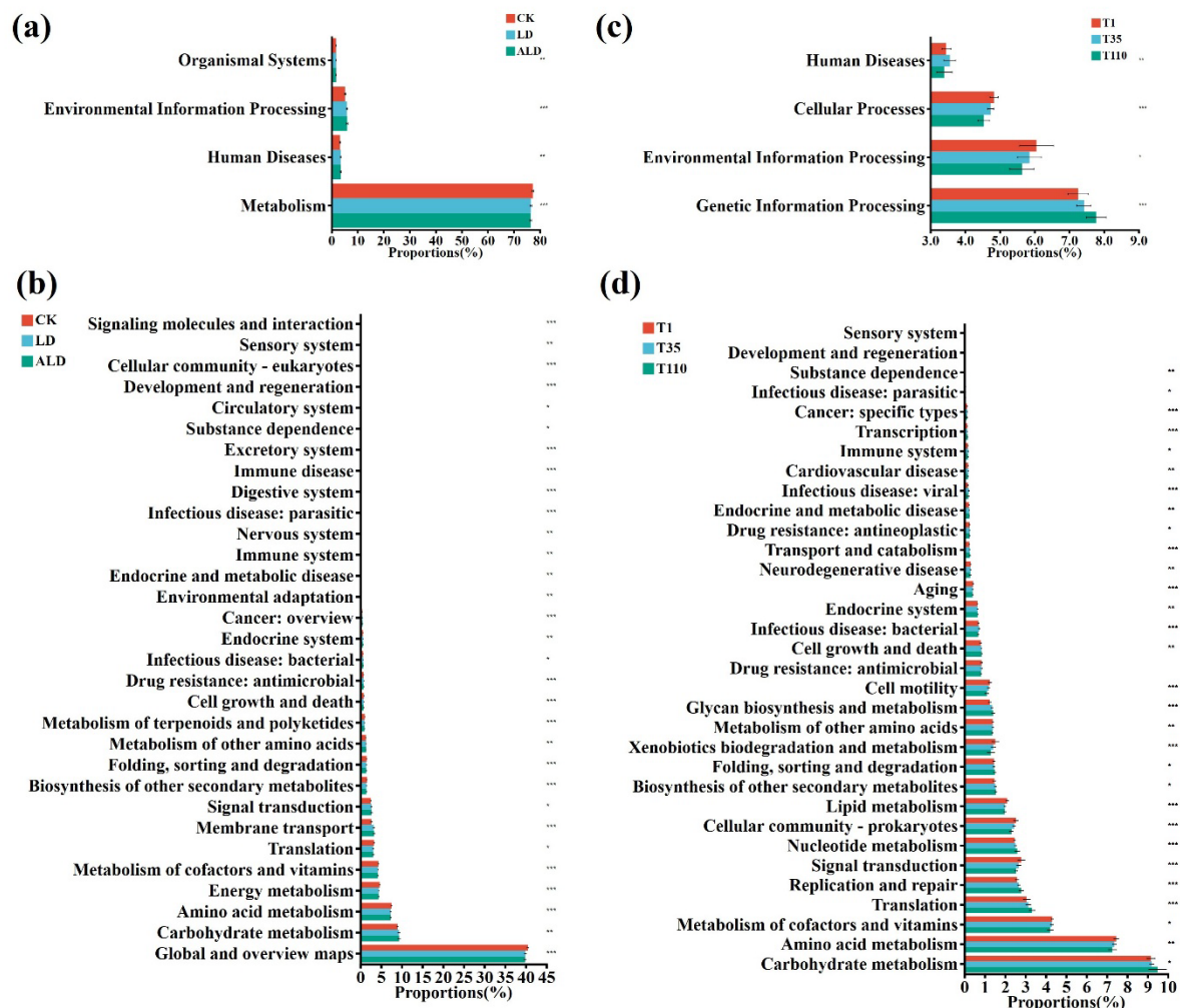
Fig. 4 Bacterial functional pathways showing significant differences at Level 1 and 2 by PICRUST2 analysis based on the KEGG database in the CK, LD and ALD groups (a and b) and three litter decomposition times (c and d) of all groups. (Control group (CK), litter decomposition group (LD), antibiotic-litter decomposition group (ALD); * P < 0.05 ; ** P < 0.01 ; *** P < 0.001 )
