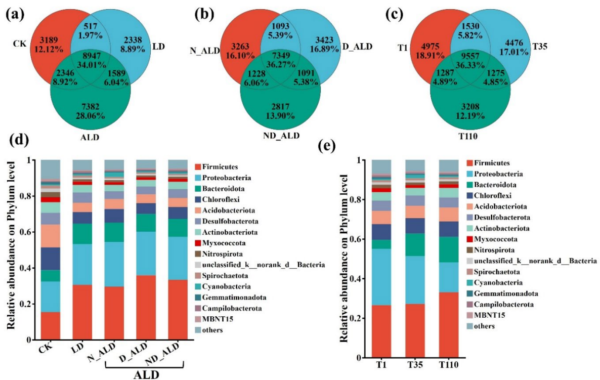
Fig. 3 Venn diagram (a-c) and the relative abundance (d and e) of bacterial communities in freshwater sediments. (Control group (CK), litter decomposition group (LD), antibiotic-litter decomposition group (ALD), norfloxacin-litter decomposition group (N-ALD), doxycycline-litter decomposition group (D-ALD), a combination of both antibiotics-litter decomposition group (ND-ALD))
