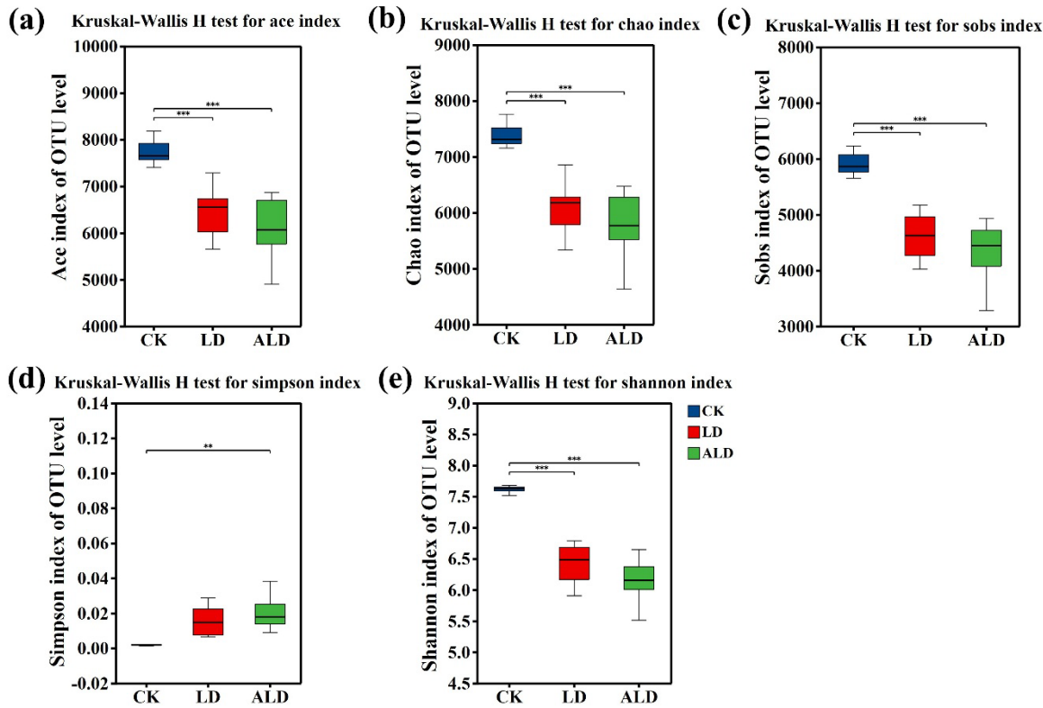
Fig. 1 Kruskal-Wallis H test bar plot of alpha diversity indices of attached bacteria in the litter decomposition group (LD), antibiotic-litter decomposition group (ALD), and control group (CK) in the sediment (* P<0.05 , ** P<0.01 )
