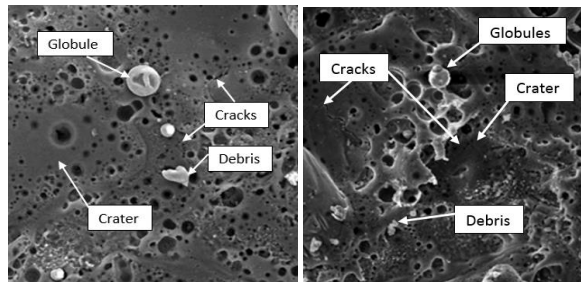
Fig. 10. Micrographs for distilled water dielectric (a) Current 6 (ampere), Pon 45 (μs); (b) Current 12 (ampere), Pon 45 (μs)
