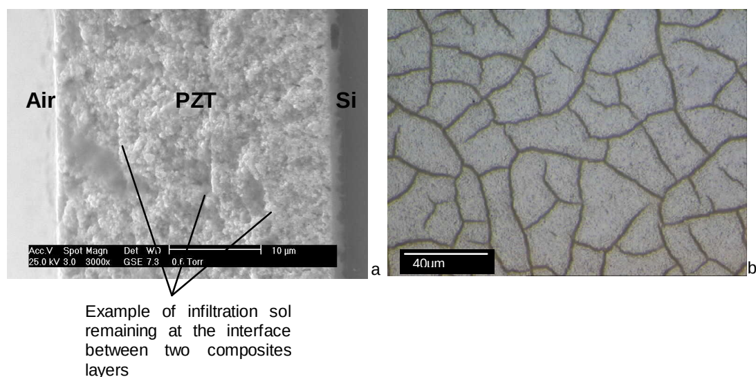
Fig 6. a) SEM micrograph of a 25 \mu\text{m} PZT thick film composed of PZT 12[C+4S]. The cross section highlights the boundary between composite layers caused by the infiltration stage, b) Light microscope image of surface of this thick film showing increase in scale of cracking.
