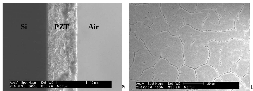
Fig 5. SEM micrograph of 10\mu\text{m} PZT thick film composed of 4[C+4S] , cross section (a), surface (b).
