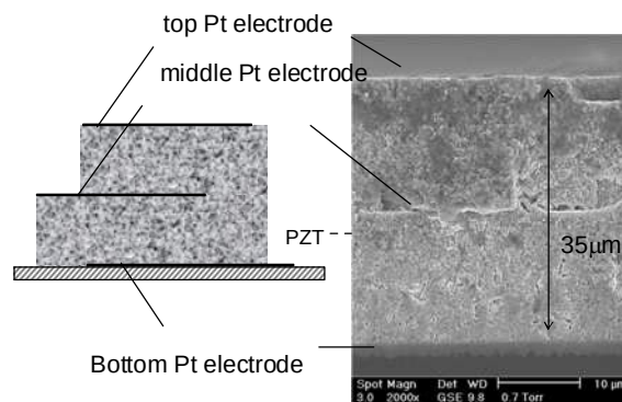
Fig 10. Schematic and SEM image of a multilayer PZT thick film 14[C+4S] with embedded electrode after the 7 th composite layers.
