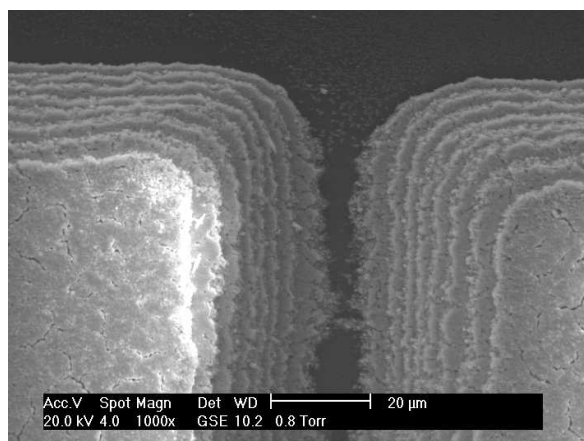
Fig. 11. SEM micrograph of a 21 \mu\text{m} PZT thick film, patterned with features at the base of 10 \mu\text{m} .
