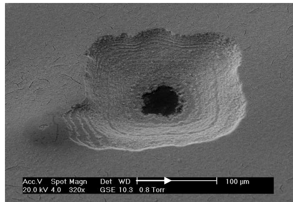
Fig 13. SEM micrograph of a 150 \mu\text{m} hole PZT in a 35 \mu\text{m} thick PZT film produced using mask with a 110 \mu\text{m} aperture. Defect near the bottom left of the hole is due to delamination of the photoresist and subsequent over etch.
