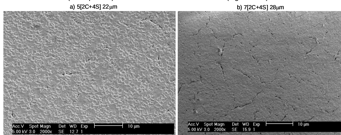
Fig 8. SEM micrograph of surface finish of the process x[2C+4S] for 2 different thicknesses of film showing a marked reproduction in cracking in comparison to x[C+4S] films. a) with 100nm of Pt sputtered the surface, b) virgin PZT surface
