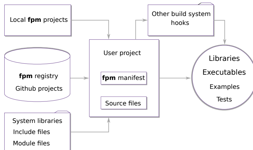
Figure 2. Fortran package manager workflow
