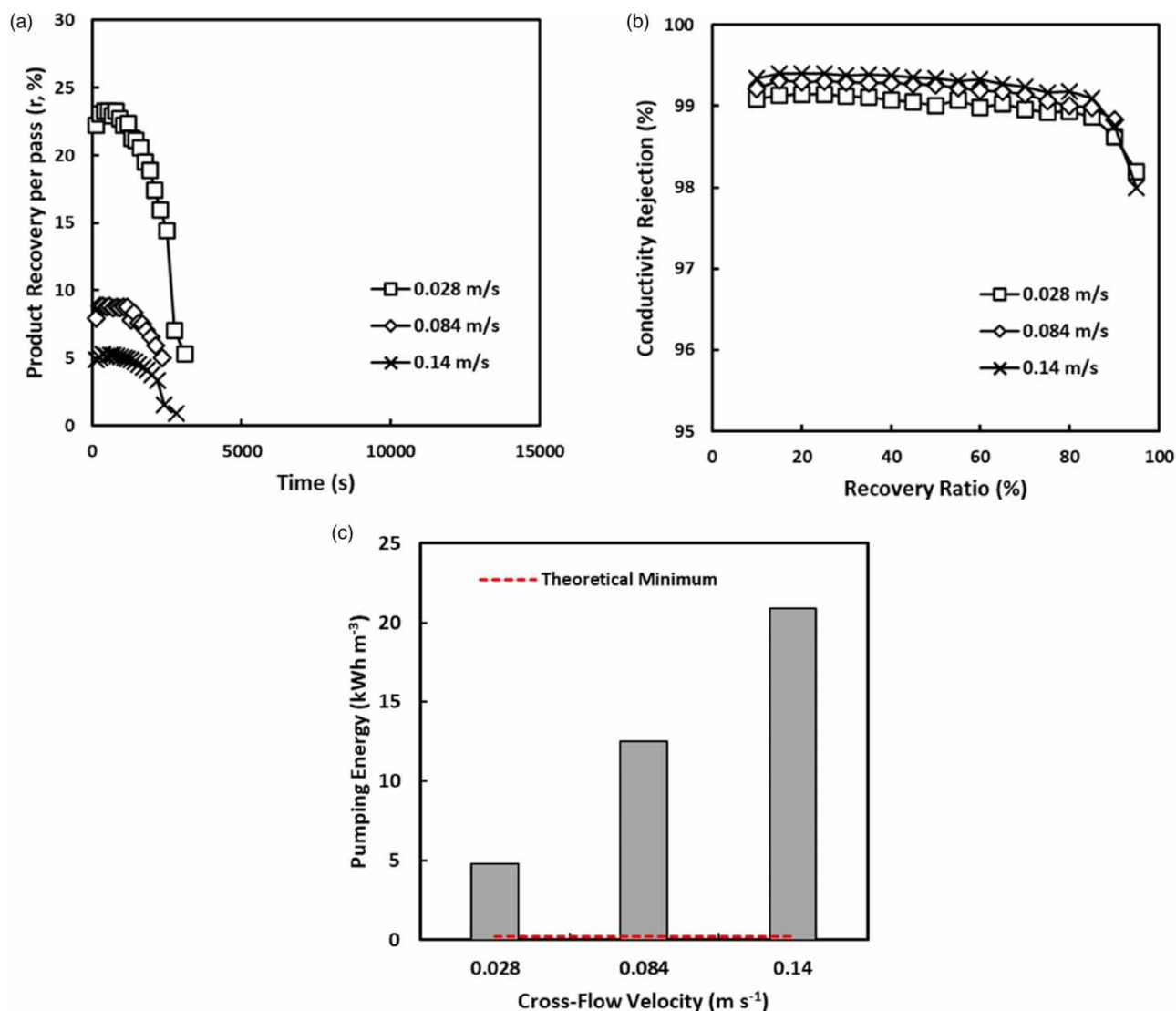
Figure 4 | Effect of the CFV on (a) RR; (b) rejection; and (c) pumping energy for a single 1812 element. Experimental conditions: feed pressure, 30 bar; 25 °C; feed volume, 10 L; RR >85%; and feed concentration 0.056 M NaCl (equivalent conductivity to blackwater).
