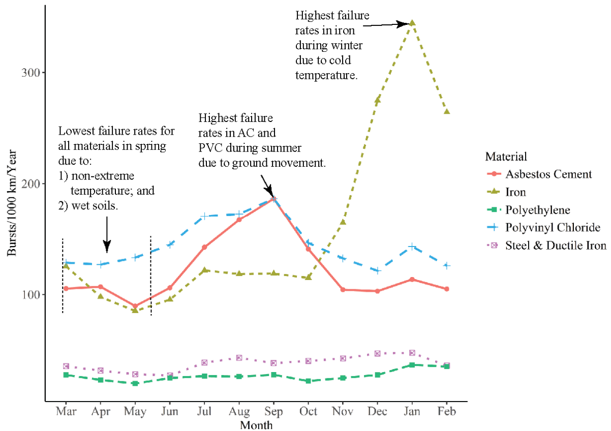
Figure 9. Summary of seasonal failure rates by material type (Utility Provider, 2018).
