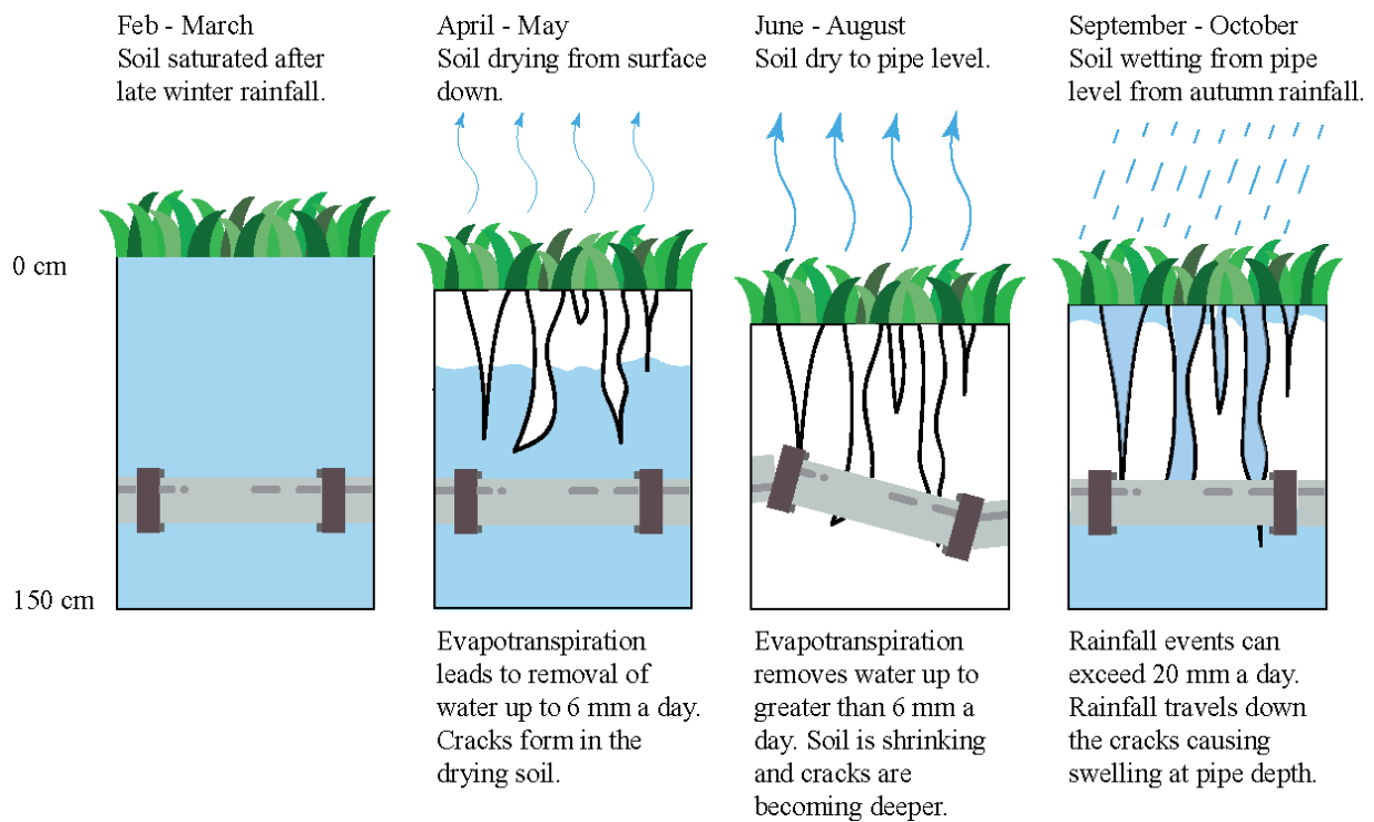
Figure 11. Seasonal shrink swell effect in clay-rich soils (after Farewell et al. , 2012, p. 10).
