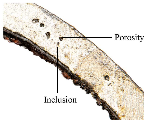
Figure 5. Porosity and inclusion defects in a cast iron pipe.
