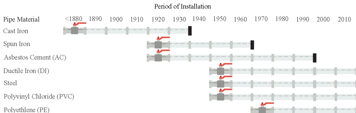
Figure 3. Approximate installation period of drinking water distribution pipe materials in the UK.
