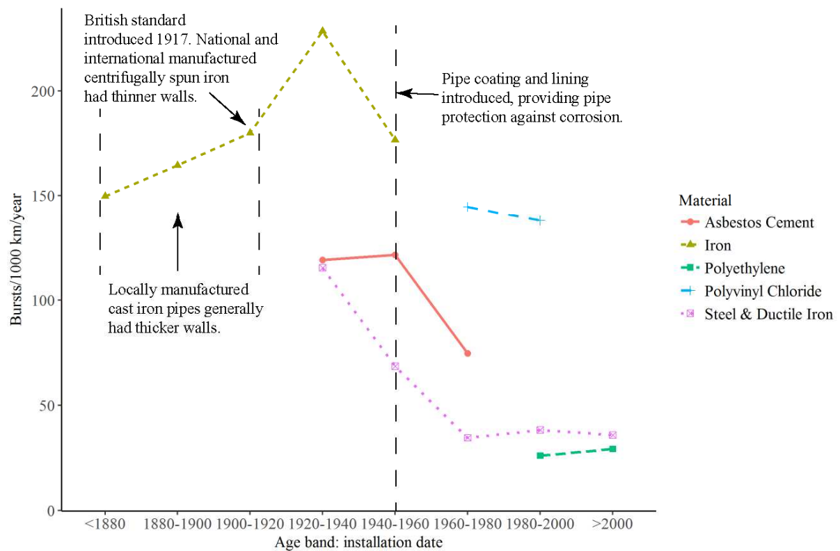
Figure 7. Summary of introduction year and successive failure rates by age by material type (Utility Provider, 2018).
