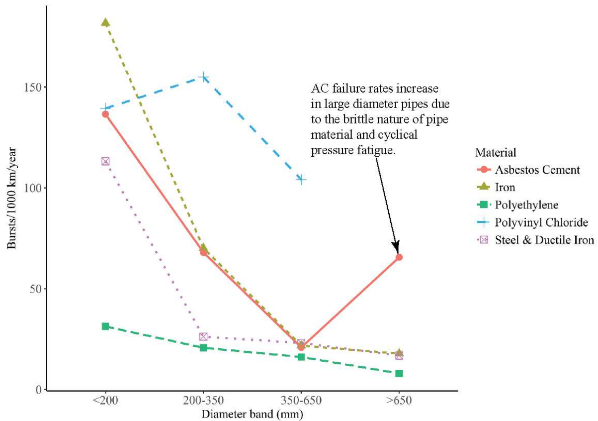
Figure 8. Summary of failure rates by diameter size and pipe material type (Utility Provider, 2018).
