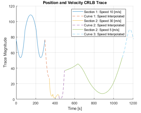
Fig. 4 Trace of the position and velocity CRLB over time
