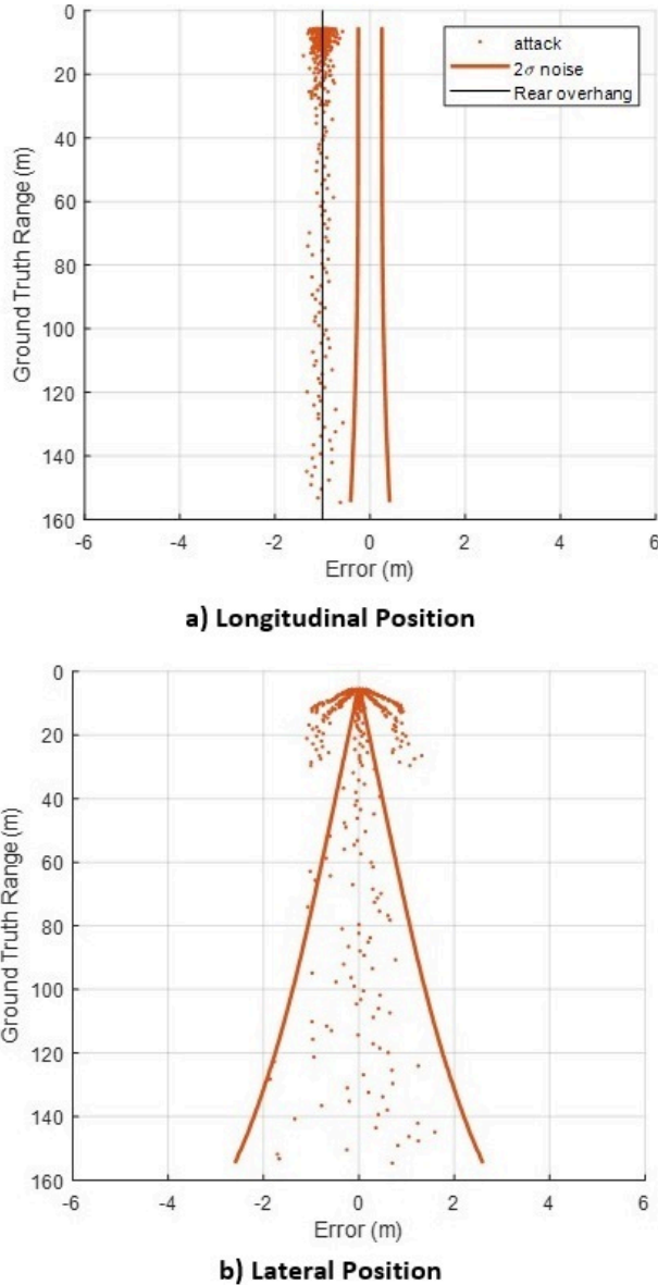
Fig. 6: Impaired detection data provided by vehicle sensors to digital twin.
