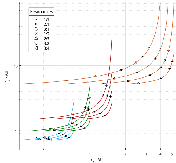
Figure 8 – Representation of the resonant orbits considered for Venus, Earth, Mars and Jupiter. v_\infty levels are 3, 5, 7 and 9 km/s.
