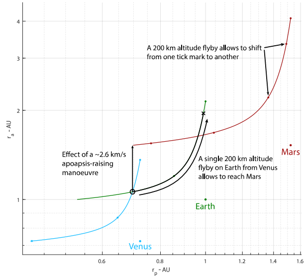
Figure 5 – Principle of a flyby on a TG. Contours plotted are for v_\infty = 5 km/s
