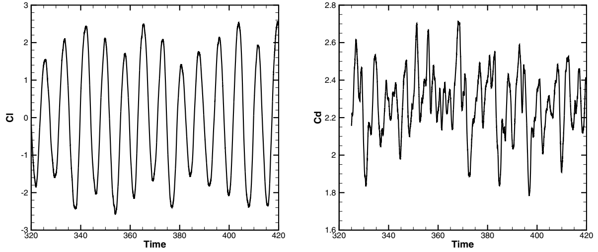
Figure 7: History of force coefficients (HR Grid)
