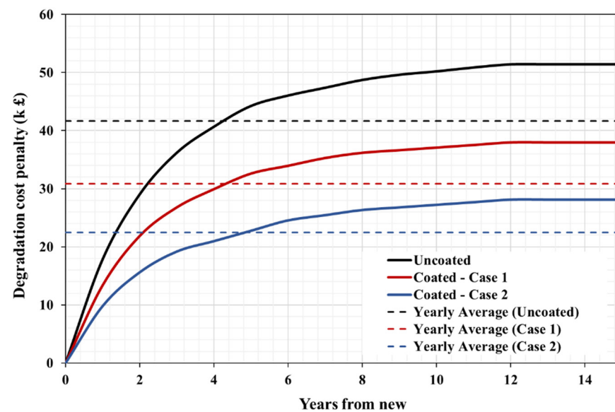
Figure 4. Fuel penalty degradation (yearly variation and average over the life of the engine).
