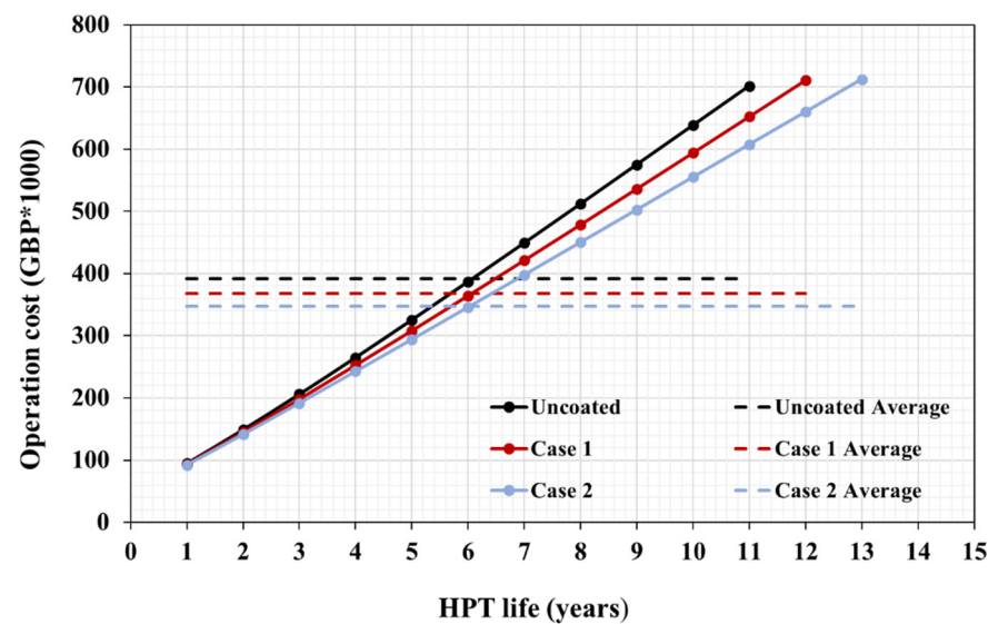
Figure 6. HPT operational cost, useful life and representative average.
