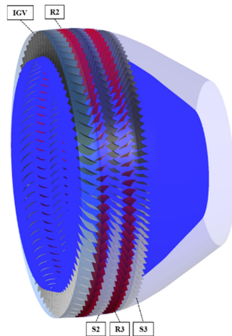
Figure 2. LPC geometry showing inlet guide vanes (IGV) and first two stages of the LPC.
