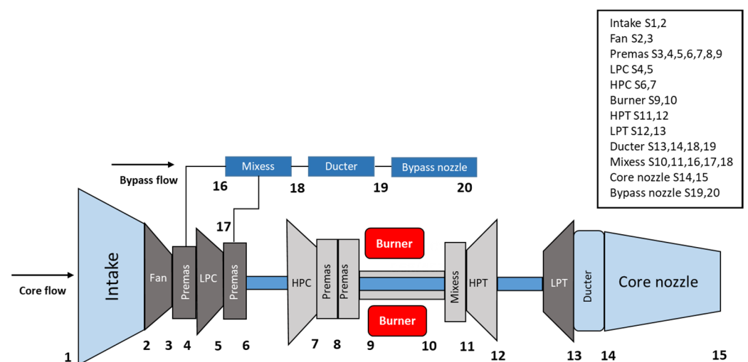
Figure 1. Research engine Turbomatch thermodynamic model showing numbered stations and component modules.
