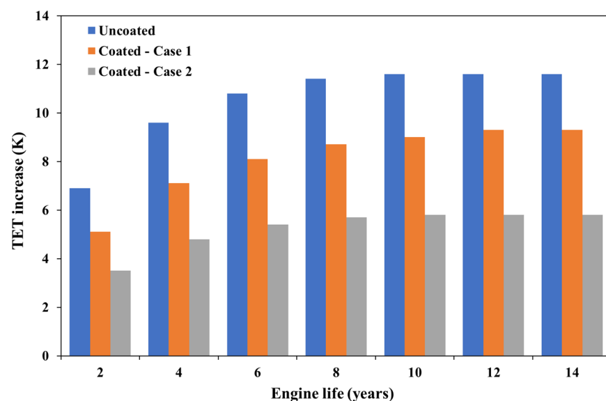
Figure 5. TET variation with time for uncoated and two LPC-coated scenarios.
