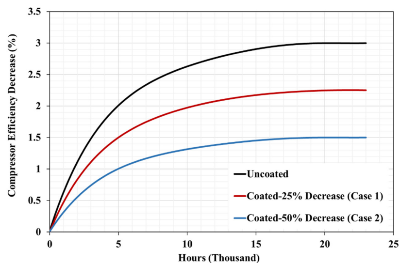
Figure 3. Performance deterioration with service hours.
