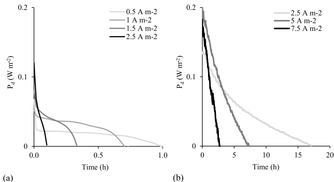
Fig. 7. Comparison of (a) low and (b) high flowrates in recycle mode until power fully extracted, at varying current draws (A m -2 ). High flowrates (concentrate and diluate at 140 mL min -1 ), low flow rates (2.5 mL min -1 concentrate/10 mL min -1 diluate). Synthetic urine concentrate, 0.004 M NaCl diluate.
