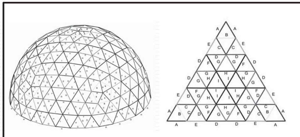
FIGURE 3. 6V Geodesic dome construction map
