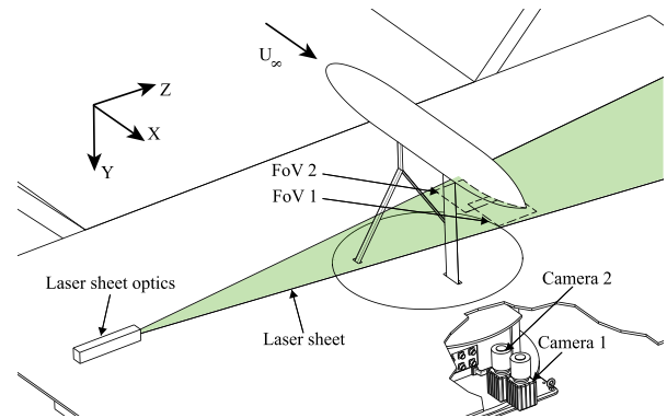
Fig. A.8. Updated stereoscopic particle image velocimetry set-up in the Delft University of Technology's OJF wind-tunnel [227].
