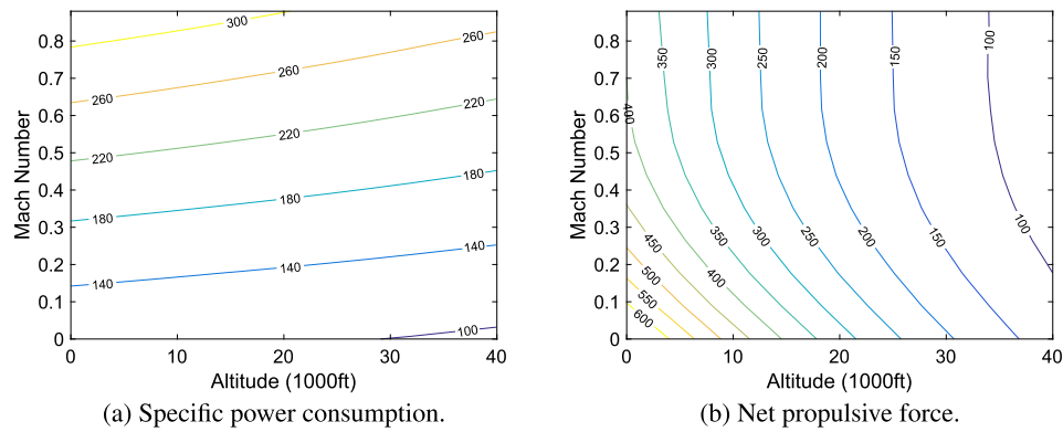
Fig. 29. Propulsor array performance in terms of (a) specific power consumption and (b) net propulsive force as a function of altitude and Mach number, retrieved from [107] 5 .
