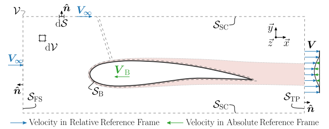
Fig. 2. Two-dimensional cutaway of a three-dimensional control volume encapsulating an aerofoil with its boundary layer development (shaded region).
