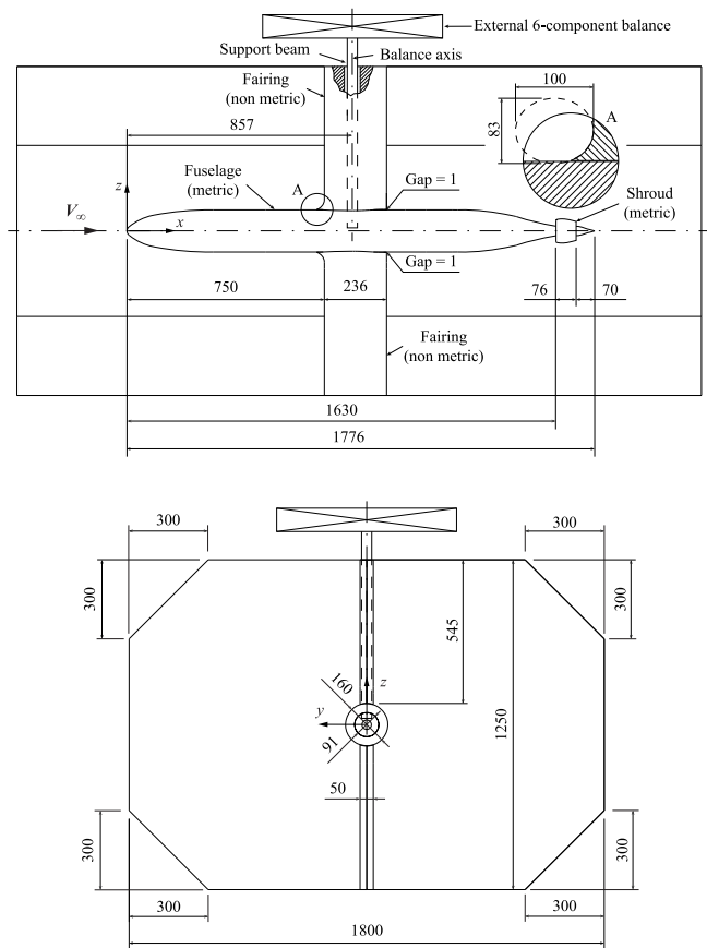
Fig. A.2. Schematic of the side and rear views of the CENTRELINE aircraft in the Low Turbulence Tunnel of Delft University of Technology.
