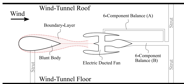
Fig. A.4. Schematic of the experimental set-up with measurements of (A) the nacelle drag and other forces and momentums, and (B) thrust, torque and other forces and momentums.
