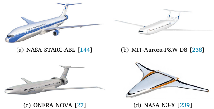
Fig. 13. BLI aircraft designs.
