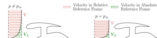
Fig. 5. Boundary layer velocity profile at the BLI propulsor's AIP (left) and its equivalent at fully-expanded isentropic conditions (right).
