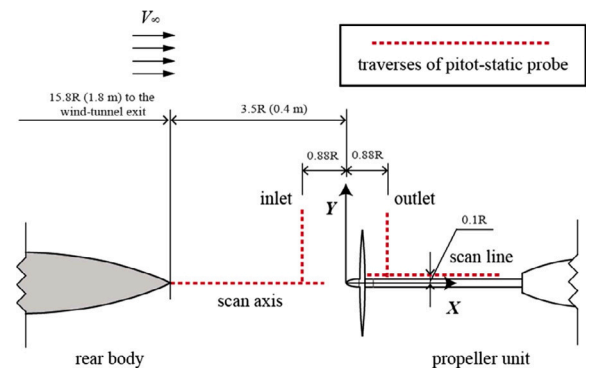
Fig. A.6. Traverse rake of pressure measurements in the Delft University of Technology's OJF wind-tunnel [220].
