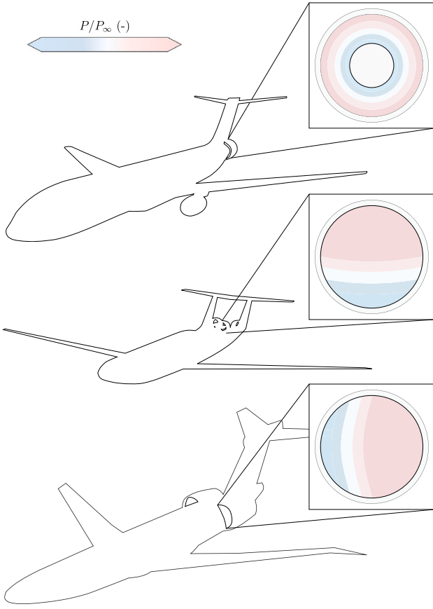
Fig. 6. Schematic of governing distortion types (normalised total pressure) for various embedded propulsion systems.
