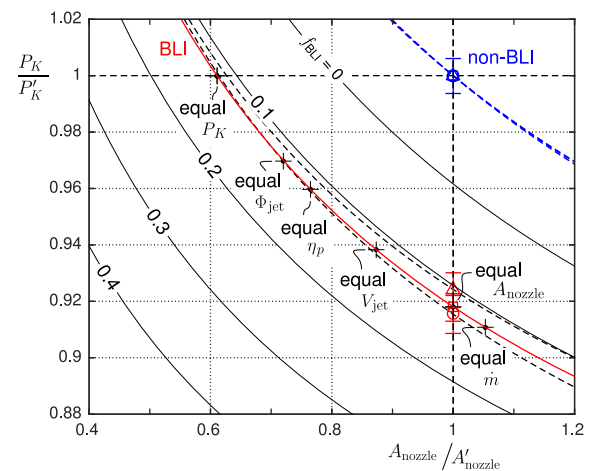
Fig. 26. Range of potential BLI propulsors with their cruise power reduction at different nozzle areas. Prime indicates non-BLI quantities and non-primed quantities relates to BLI.
