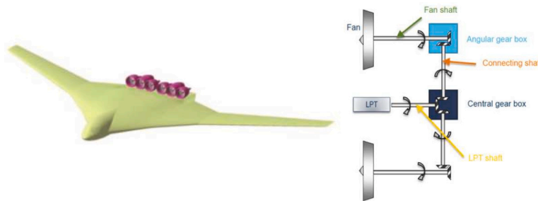
Fig. 27. Schematic of the DisPURSAL architecture and power transmission. Source: Modified from Ref. [49].
