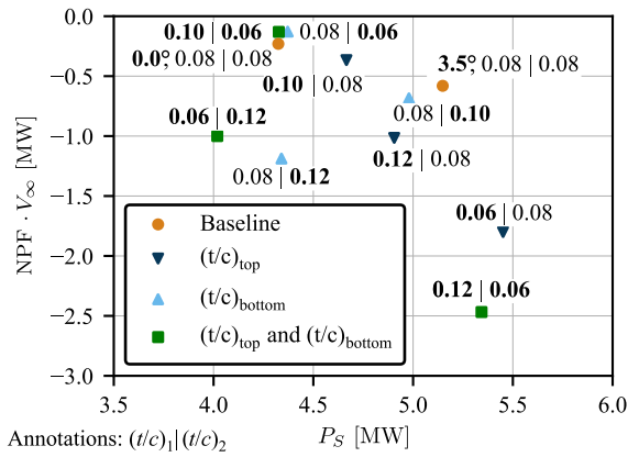
Fig. 18. Comparison of the aero-propulsive performance between the baseline and geometries with variations in thickness-to-chord ratios ( t/c ), from Ref. [157].
