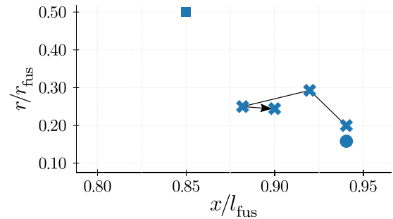
Fig. 23. Positions of the STARC-ABL (●), CENTRELINE (✕) with its evolution (→) and DisPURSAL (■) relative to their fuselage dimensions.
