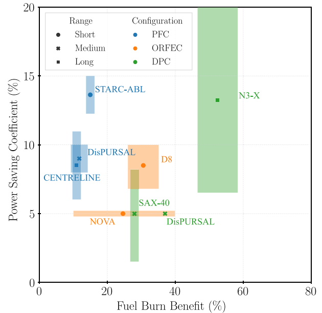
Fig. 31. Boundary layer ingestion benefits in power savings coefficient, relative to the concepts' podded equivalent, and technology and synergistic benefits in fuel burn, relative to their tube-and-wing reference.
