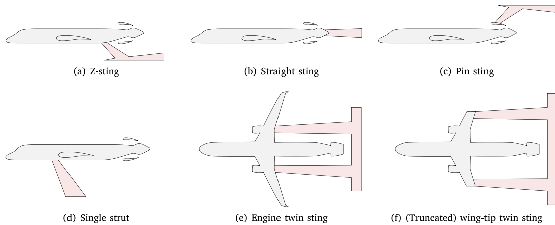
Fig. A.3. Schematics of wind-tunnel model supports applicable for powered boundary layer ingesting aircraft.
