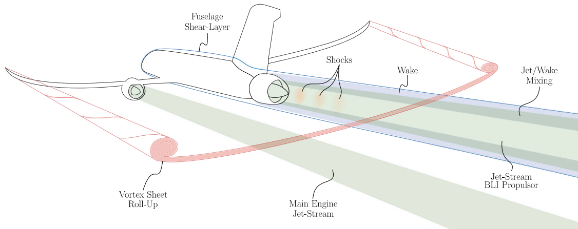
Fig. 8. Flow features around a propulsive fuselage aircraft.
