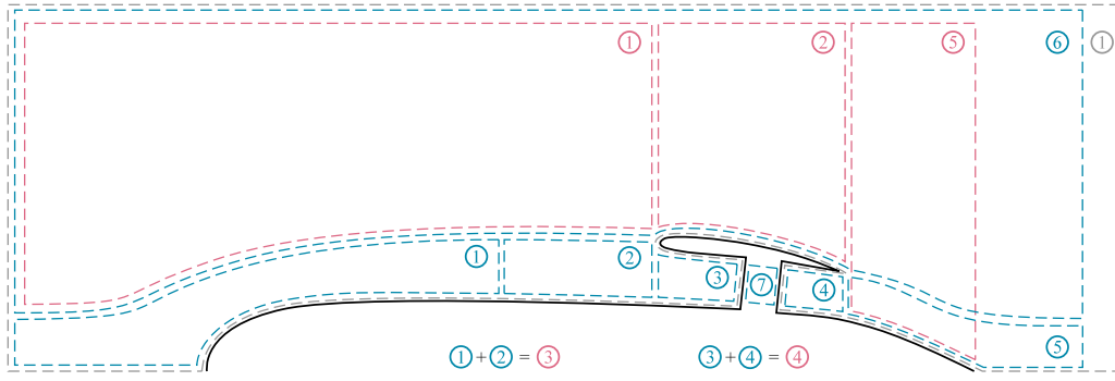
Fig. 4. Control volume divisions based on Habermann et al. [32] ① to ⑤, Sanders [31] ① to ⑦, and Gray [62] ①.
