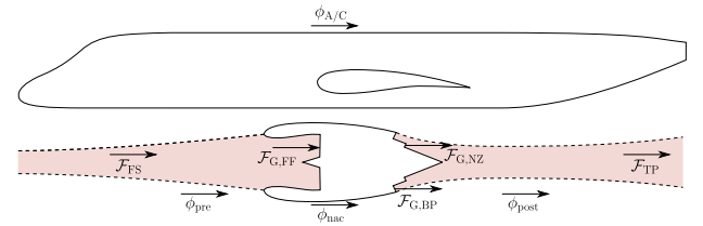
Fig. 3. Forces decomposition on stream-tubes, nacelle and airframe based on the thrust-drag accounting.
