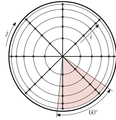
Fig. 7. Rake and pressure probes arrangement with a fictitious critical sector of 60°. Source: Remastered from Ref. [79].
