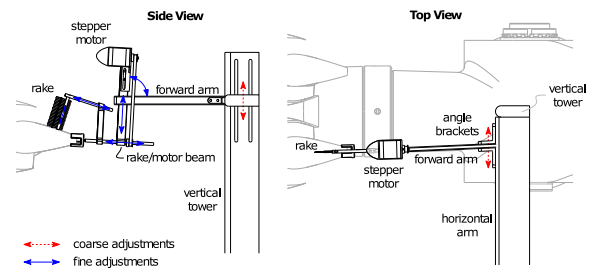
Fig. A.5. Rotating rake of pressure measurements in the NASA Langley's 14 × 22 wind-tunnel [109].
