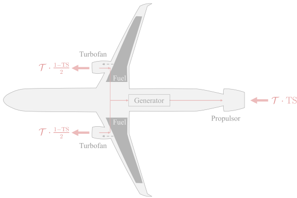
Fig. 15. Propulsive fuselage and thrust-split concepts.
