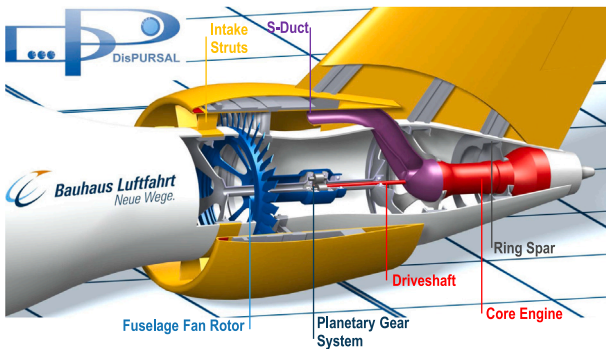
Fig. 20. Cutaway view of the rear-mounted DisPUSAL propulsion system, from Ref. [260].
