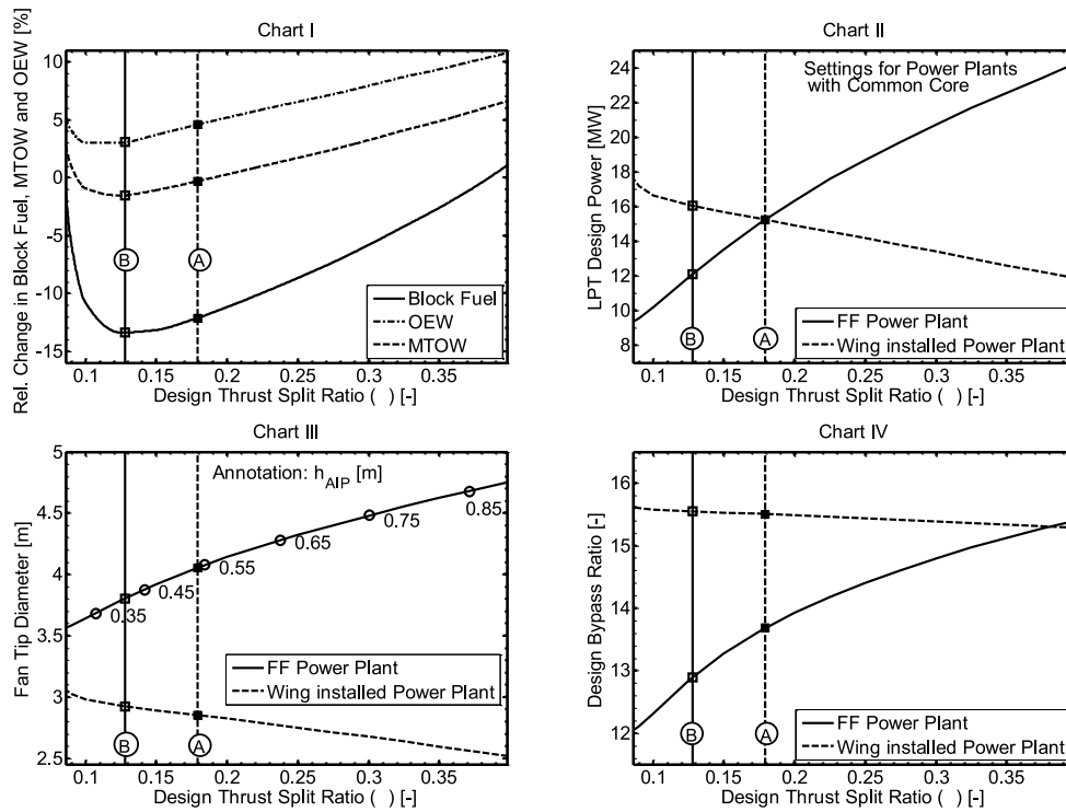
Fig. 21. Characteristics of thrust-split optimality study for two designs (A and B), FF denoting fuselage-fan, i.e. BLI propulsor, coupled to two under-wing engines for a design range of 4800 nmi carrying 340 PAX with a cruise segment flown at M0.82 and FL350. Source: Retrieved from Ref. [148].
