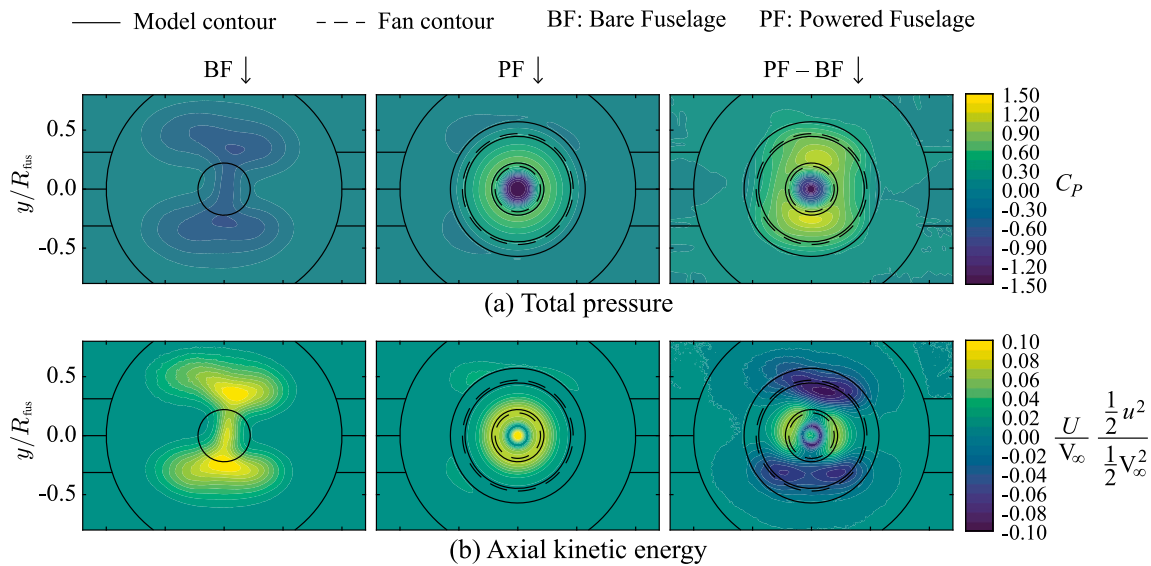
Fig. 19. Measured total pressure and axial kinetic energy in the wake-plane field of view for the bare fuselage, powered fuselage and their difference, from Ref. [180].
