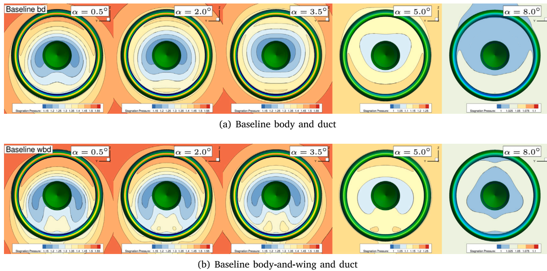
Fig. 17. Computed total pressure contours at AIP for different angles of attack highlighting the down-wash effects, Ref. [161].
