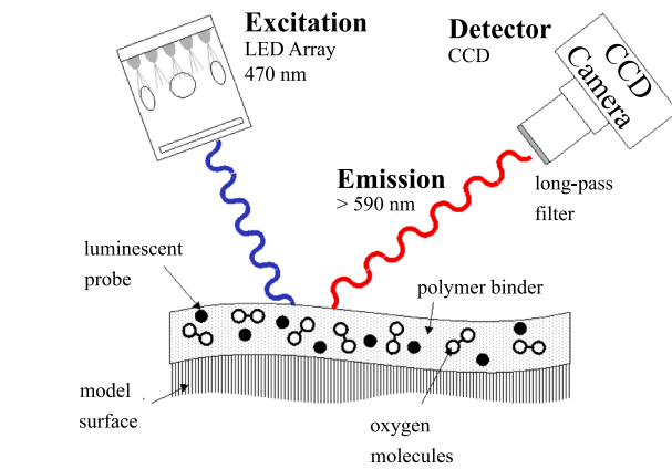
Fig. A.7. Pressure-sensitive paint, light and camera system in the ARA 9 × 8 Transonic Wind-Tunnel [234].
