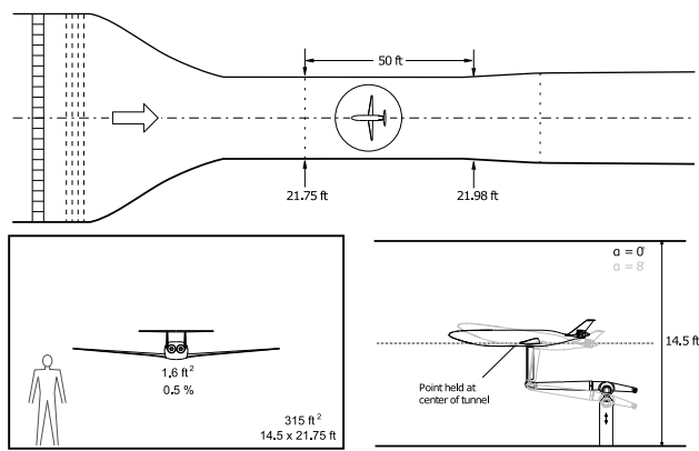
Fig. A.1. Schematic of the top, rear and side views of the MIT D8 aircraft in the NASA Langley's 14 × 22 wind-tunnel.
