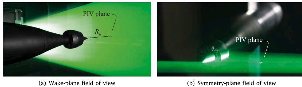
Fig. 12. Stereoscopic particle image velocimetry measurement set-up, from Ref. [180].
