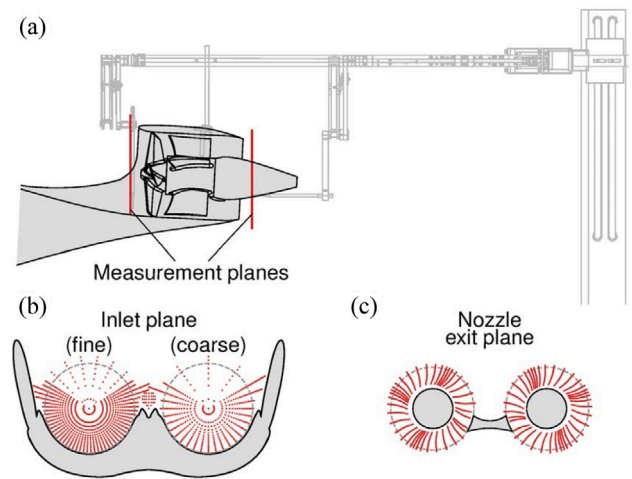
Fig. 10. Experimental (a) model-mounted survey systems and measurement plane locations, (b) measurement grids for BLI inlet and (c) nozzle exit surveys, from Ref. [76].
