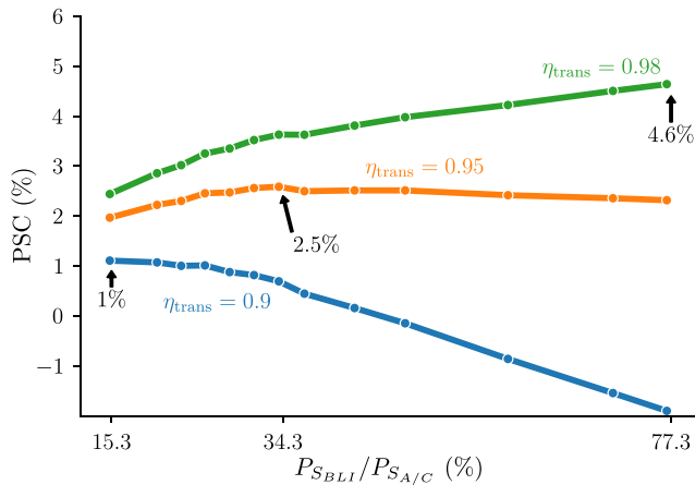
Fig. 16. Overall aircraft PSC at cruise versus the fraction of shaft power used for BLI under different transmission efficiencies, \eta_{trans} . Source: Adapted from Ref. [145].
