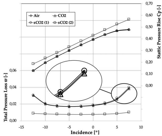
Fig. 4. Static pressure rise and total pressure loss for atmospheric air and atmospheric/supercritical CO 2 cascades.
