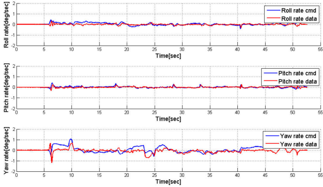
Fig. 17 Result of the flight test (angular velocity)
