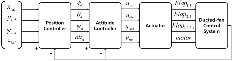
Fig. 6 Diagram of the control system of the ducted-fan UAV
