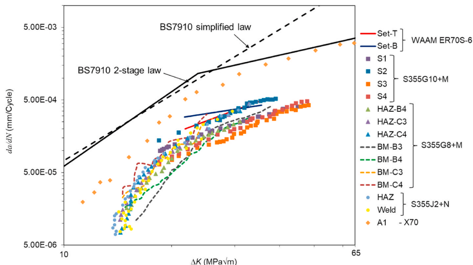
Fig. 10. Comparison of the upper bound CFCG trends for ER70S-6 WAAM specimens with BS7910 curves and the literature data on structural steels.
