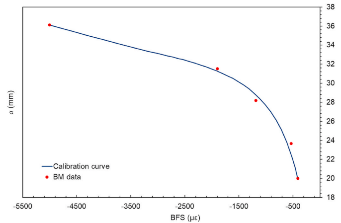
Fig. 6. Crack length vs. BFS values for CT-HB specimen tested in seawater, and the comparison with the beach marking data.
