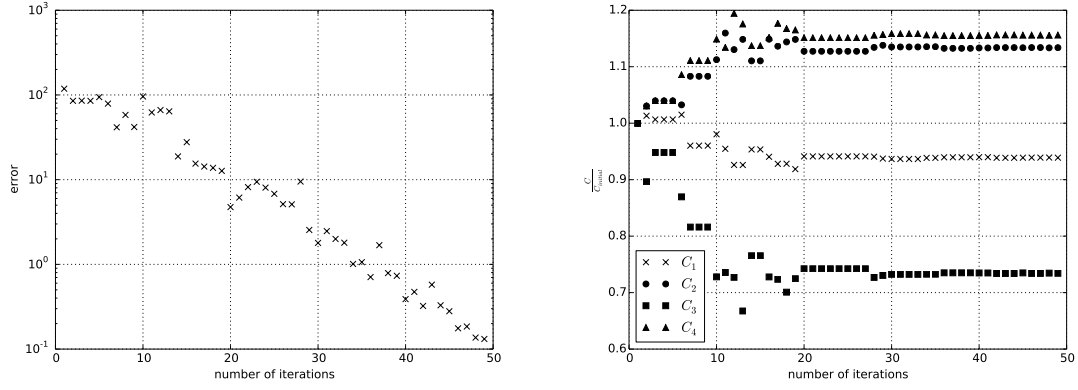
Figure 2: Rate of convergence of optimization process. Left-hand side plot shows error as defined by Eq. 15 as a function of number of iterations. The second plot shows relative change in C_1 – C_4 parameters being optimized.
