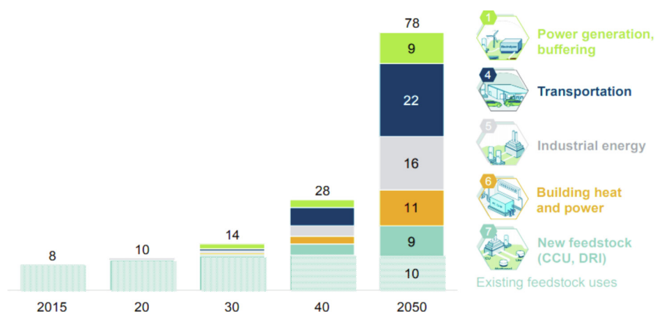
Figure 9. Projected increase in hydrogen demand by 10-fold in 2050 (The role of green hydrogen in global decarbonization 2018).
