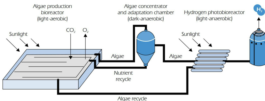
Figure 7. The photobiological H_2 production concept (Hydrogen projects database 2021).
