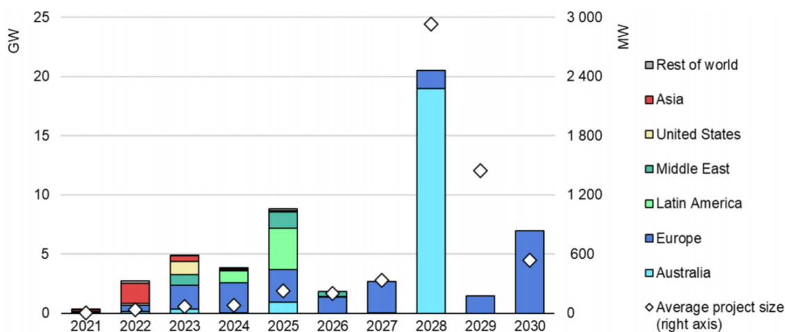
Figure 6. 2021-2030 New electrolyser capacity installed as a result of ongoing or planned projects (Hydrogen projects database 2021).
