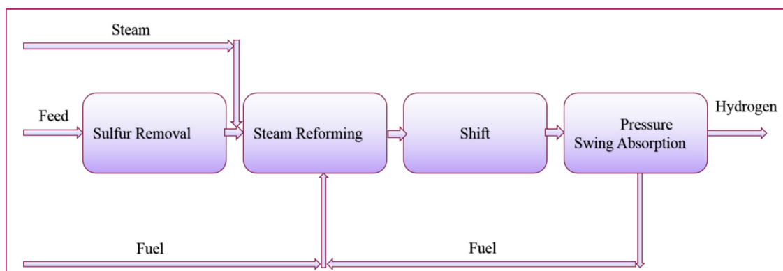
Figure 3. The steam methane reforming process schematic presentation.
