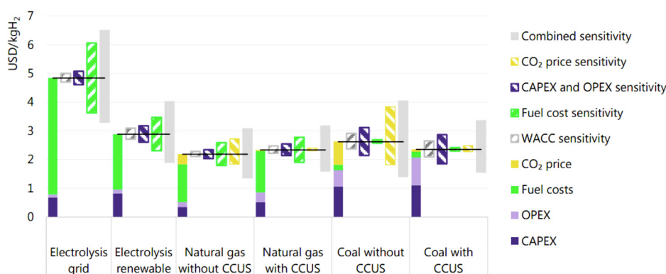
Figure 11. Estimated costs of hydrogen production in 2030 for various technology options. Renewable electricity price = USD 40/MWh at 4,000 full load hours in best locations; sensitivity analysis based on \pm 30\% variation in OPEX, CAPEX, and fuel costs; \pm 8\% change in default WACC; and a USD40/tCO 2 price variation to USD0/tCO 2 and USD100/tCO 2 levels (Hydrogen projects database 2021).
