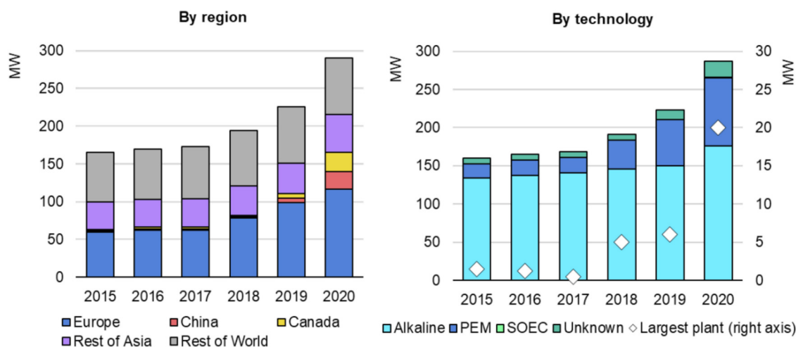
Figure 5. Global installed electrolysis capacity by technology and region (Hydrogen projects database 2021).
