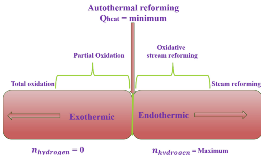
Figure 4. Operating conditions for Partial oxidation, steam reforming, and autothermal reforming (Lee, Lee and Hwang, 2019).
