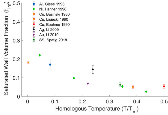
Fig. 4. Saturated wall volume fraction of PSB as a function of homologous temperature for different FCC metals (Basinski et al., 1980; Giese and Estrin, 1993; Lisiecki and Weertman, 1990; Hahnner et al., 1998; Boehme et al., 1990; Li et al., 2009; Spätig et al., 2018; Li et al., 2010).
