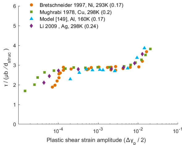
Fig. 18. Cyclic stress-strain response of Ni, Cu, Ag, and Al single crystals at the same homologous temperature, the y-axis is normalized with the bow-out stress (Brown, 2006). d_{\text{struc}} was estimated as the PSB wall spacing computed from TEM (Ashraf and Castelluccio, 2021).
