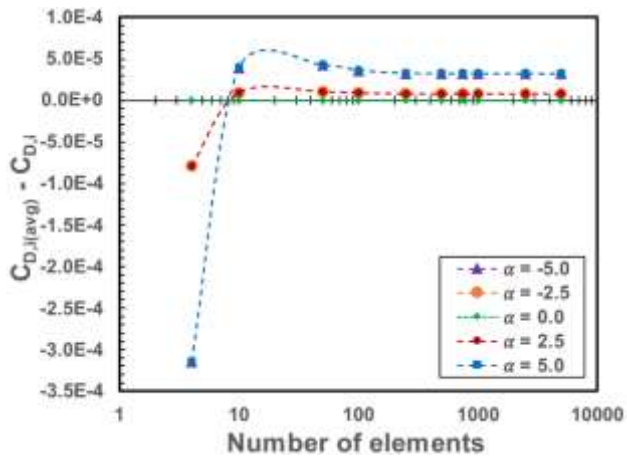
Fig. 2: NACA0012, OGE residuals C_{D,i}
