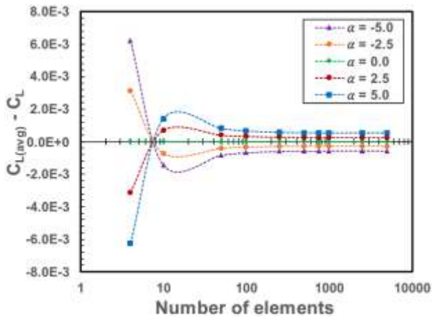
Fig. 1: NACA0012, OGE residuals C_L
