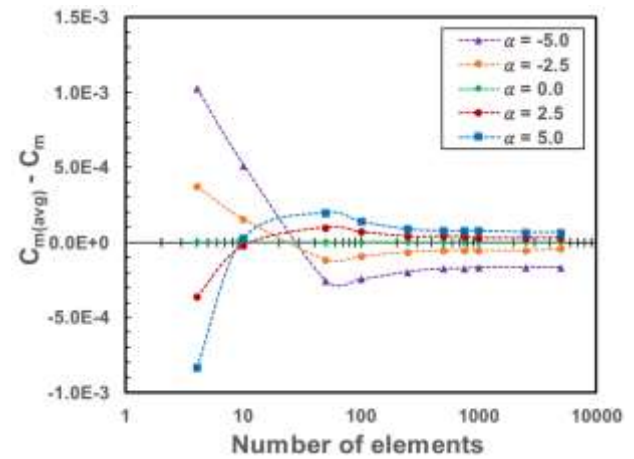
Fig. 6: NACA0012, IGE ( h/c=0.4 ) residuals C_m
