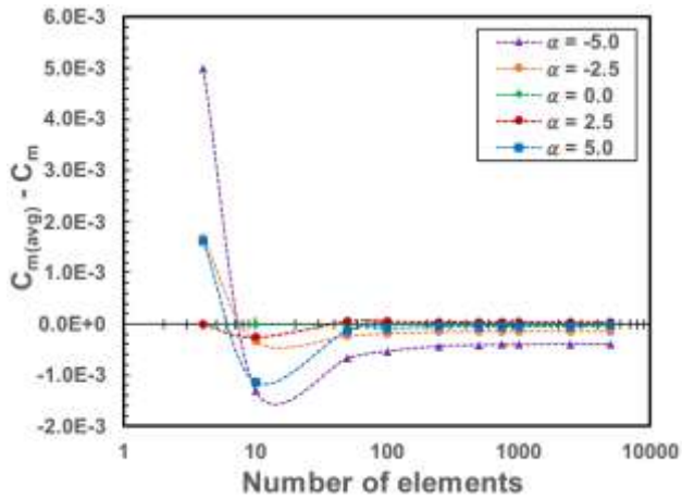
Fig. 3: NACA0012, OGE residuals C_m
