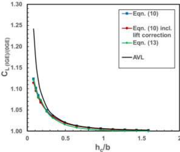
Fig. 9: NACA0012, K_3
