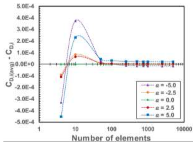
Fig. 5: NACA0012, IGE ( h/c=0.4 ) residuals C_{D,i}
