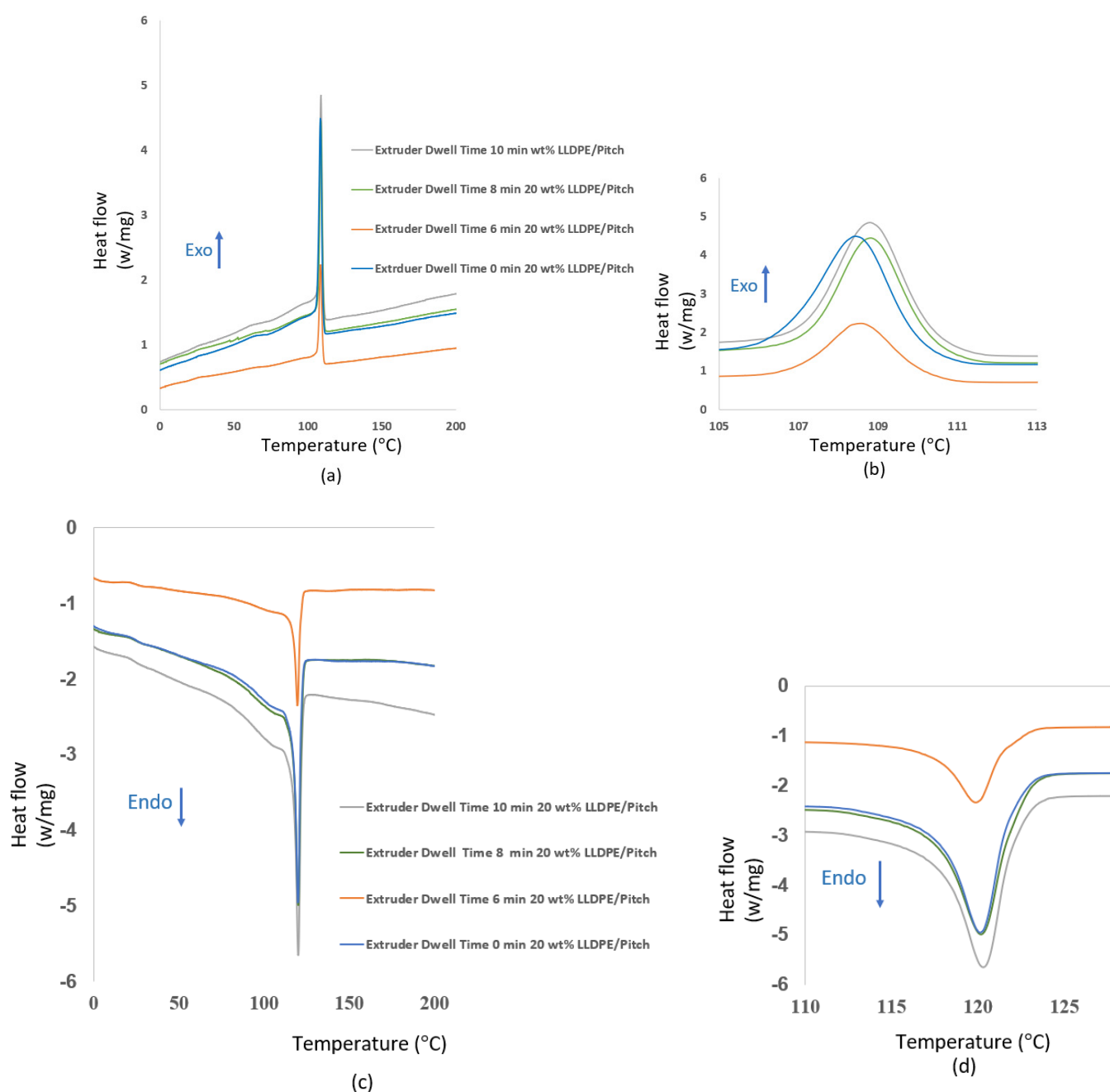
Figure 6. (a,b) Exothermic heat flow vs. temperature for crystallisation of LLDPE/MP sample and (c,d) endothermic heat flow for melting of LLDPE/MP sample. Four different extrusion dwell times. (Enthalpy of crystallisation, \Delta H_c , and enthalpy of fusion, \Delta H_m , are the areas under the respective curves).
