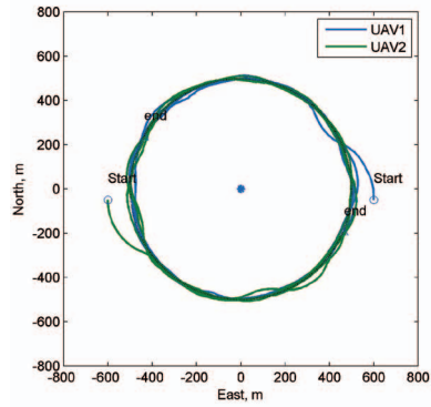
(b) Relative trajectories of UAVs
