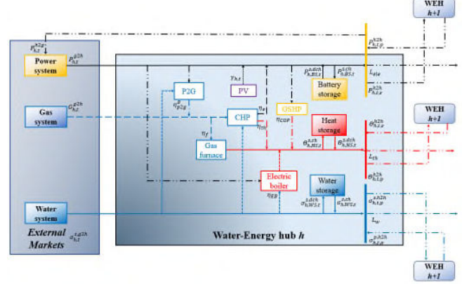
Fig. 3. Structure of the proposed IWEH.
