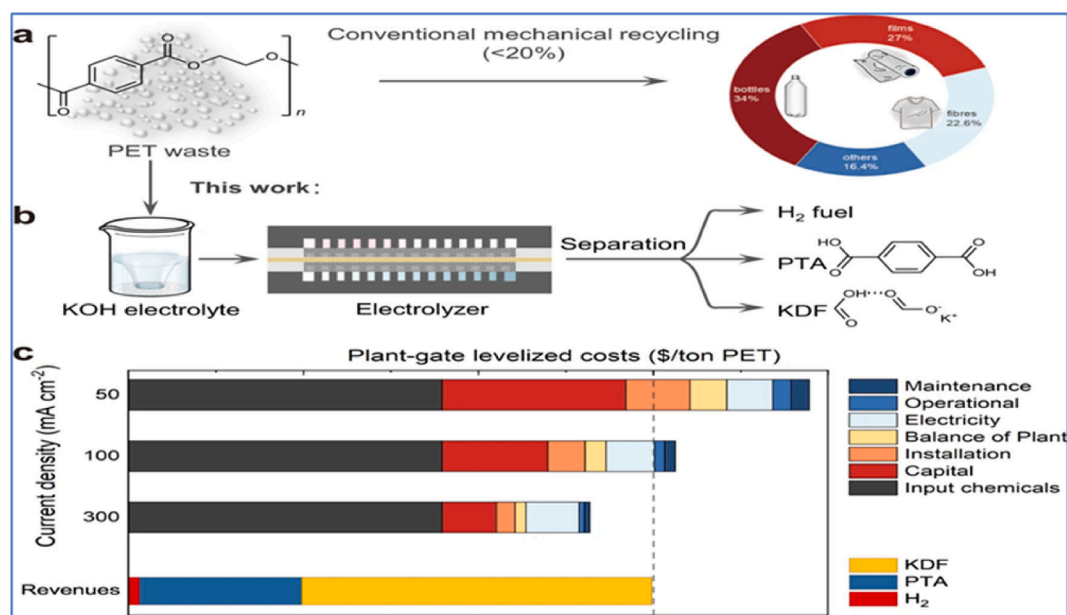
Fig. 2. (a) Conventional route for PET recycling. (b) Electrocatalytic PET upcycling to commodity chemicals and H 2 fuel (Route I). (c) Techno-economic analysis (TEA) of Route I at different current density. Copyright 2022, nature communications [127].
