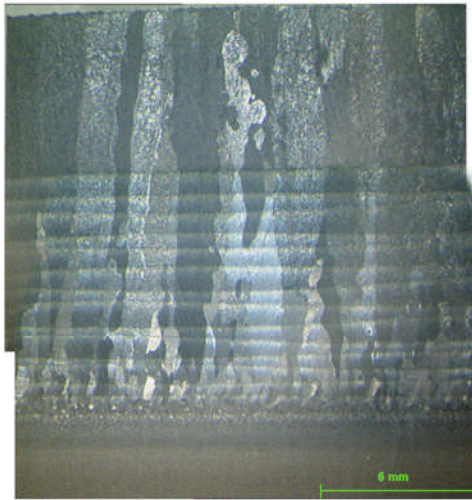
Fig. 3 Photograph of pulse GTAW deposition Ti6Al4V with I_p/I_b ratio at 7.7, average current 99A, travel speed 0.27m/min, wire feed speed 1.6m/min shows holes and humps caused by high arc pressure
