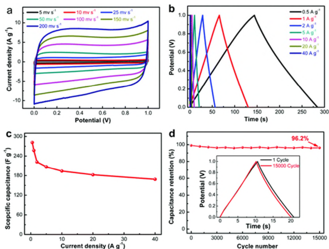
Fig. 6 Electrochemical performance characteristics of CsCNBs*4 measured in a two-electrode system using 6 M KOH as the electrolyte. (a) CV curves obtained at various scanning rates ranging from 5 mV s -1 to 200 mV s -1 ; (b) GCD curves obtained at different
