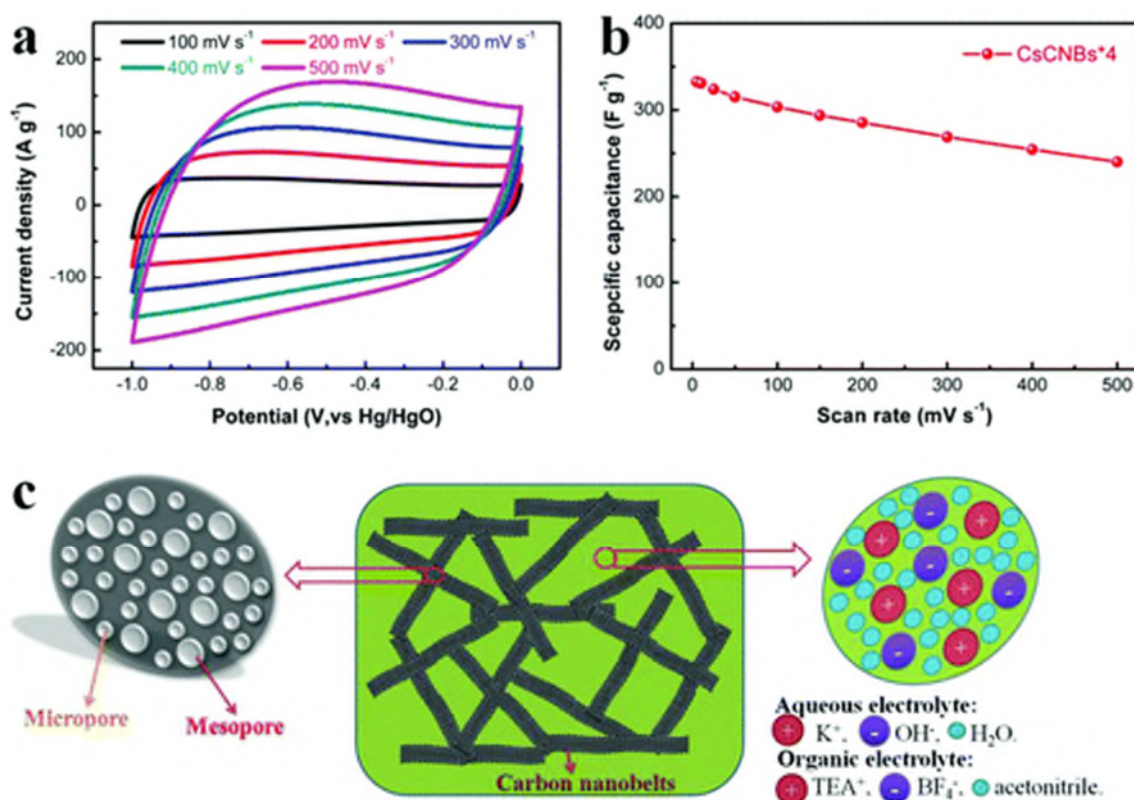
Fig. 8 CsCNBs*4 measured in a three-electrode system using 6 M KOH electrolyte: (a) CV curves obtained at various scanning rates ranging from 100 to 500 mV s -1 ; (b) specific capacitances at different potential scanning rates. (c) Schematic illustration of the electrode prepared from CsCNBs*4.
