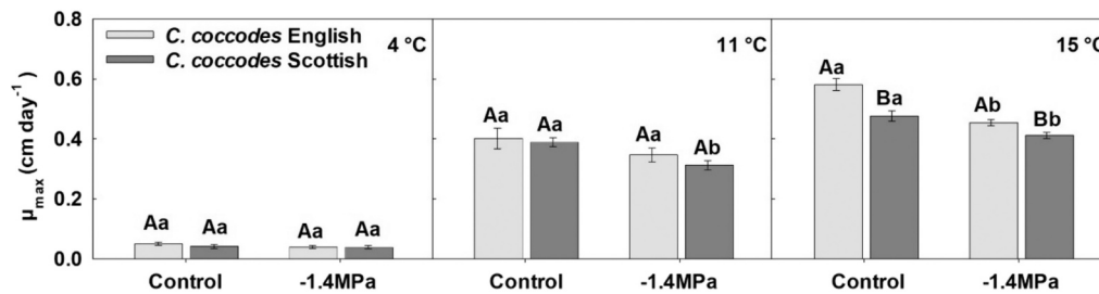
Fig. 5. Effect of temperature (4, 11, 15 °C) and water potential [Control (−0.7 MPa), −1.4 MPa] on maximum growth rate ( \mu_{max} ) of C. coccodes strains from England and Scotland on soil extract agar media. Data shows means of five replicates with standard error bars of the means. Different capital letters indicate significant differences between isolates (English black dot and Scottish black dot) at each specific temperature and water potential. Different lower-case letters indicate significant differences between water potentials at each temperature and isolate (Wilcoxon, p -value<0.05).
