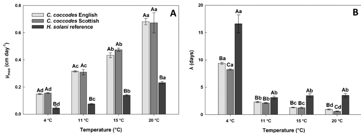
Fig. 7. Effect of temperature (4, 11, 15, 20 °C) on maximum growth rate ( \mu_{max} ) (A) and lag time ( \lambda ) (B) of C. coccodes strains from England and Scotland and H. solani on potato-based media. Data shows means of 5 replicates with standard error bars of the means. Different capital letters indicate significant differences between isolates (English black dot and Scottish black dot) at each specific temperature. Different lower-case letters indicate significant differences between temperatures for each isolate (Wilcoxon, p -value<0.05).
